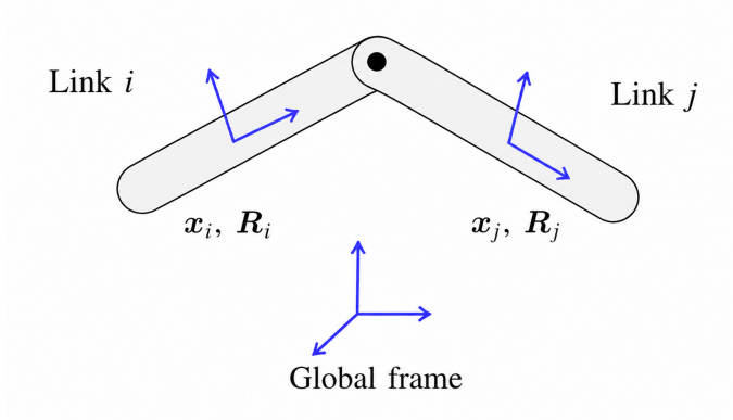
Figure 4.1: Two rigid bodies connected by a holonomic joint in maximal coordinates. Adapted from [?].
