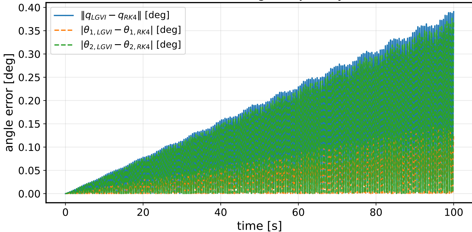
Forced Acrobot angle trajectory error
