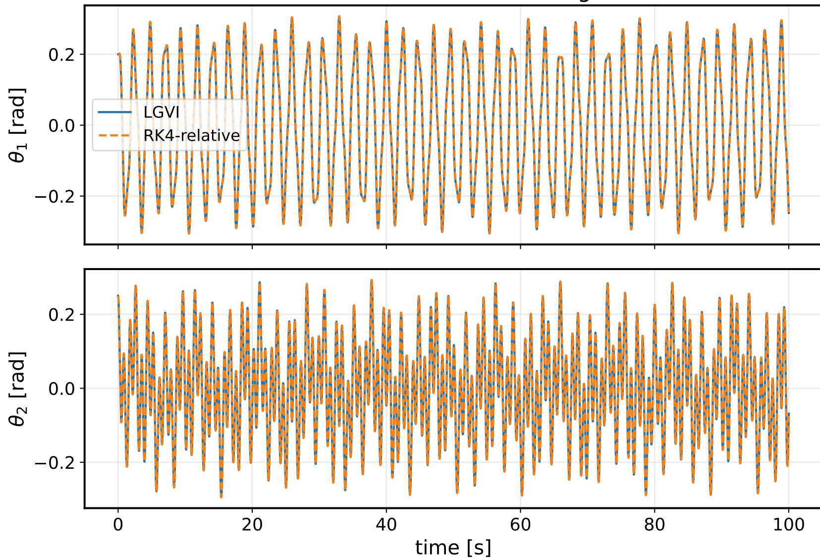
Forced Acrobot relative angles
