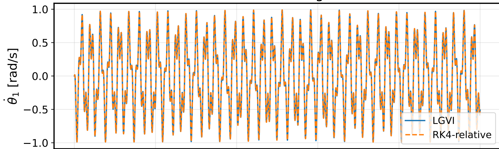
Forced Acrobot relative angular velocities
