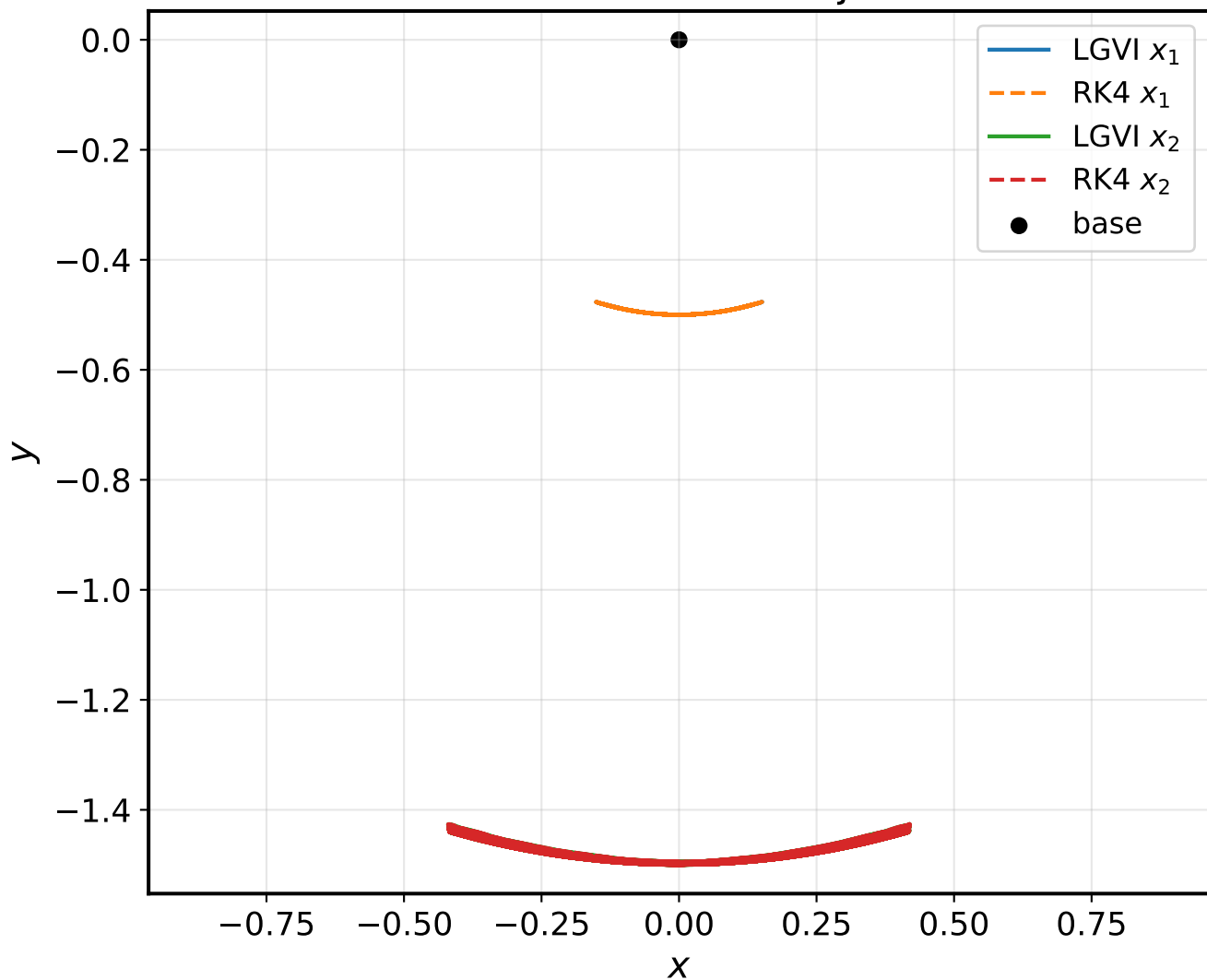
Forced Acrobot COM trajectories
