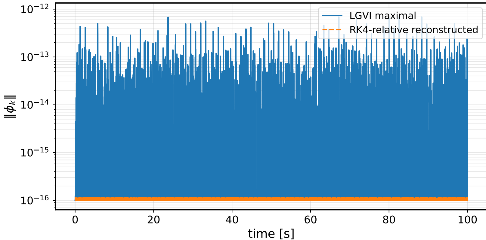
Forced Acrobot constraint residuals
