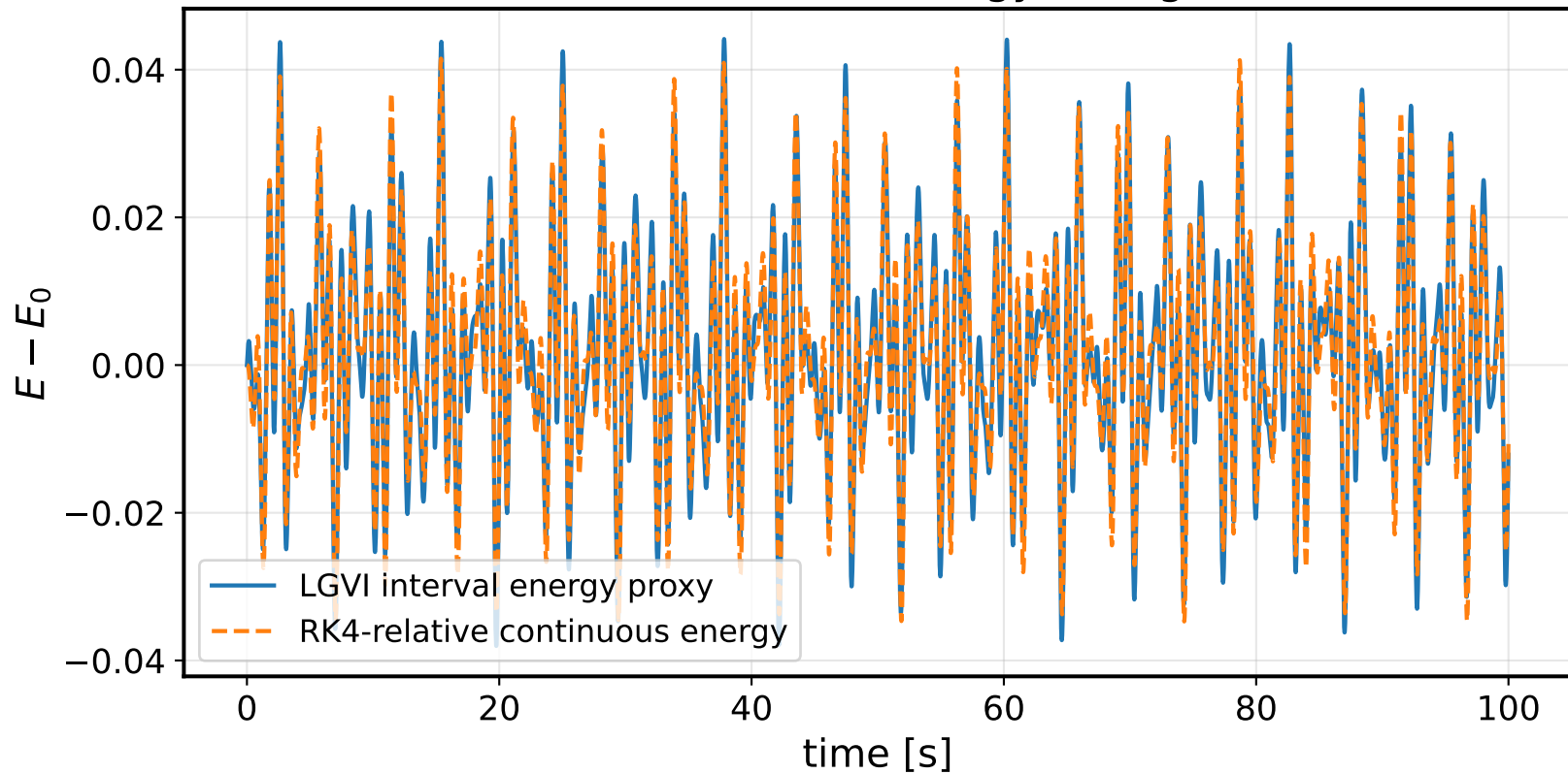
Forced Acrobot energy change
