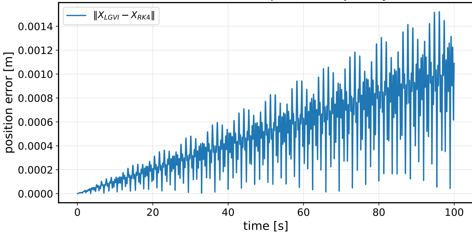
Forced Acrobot maximal position trajectory error
