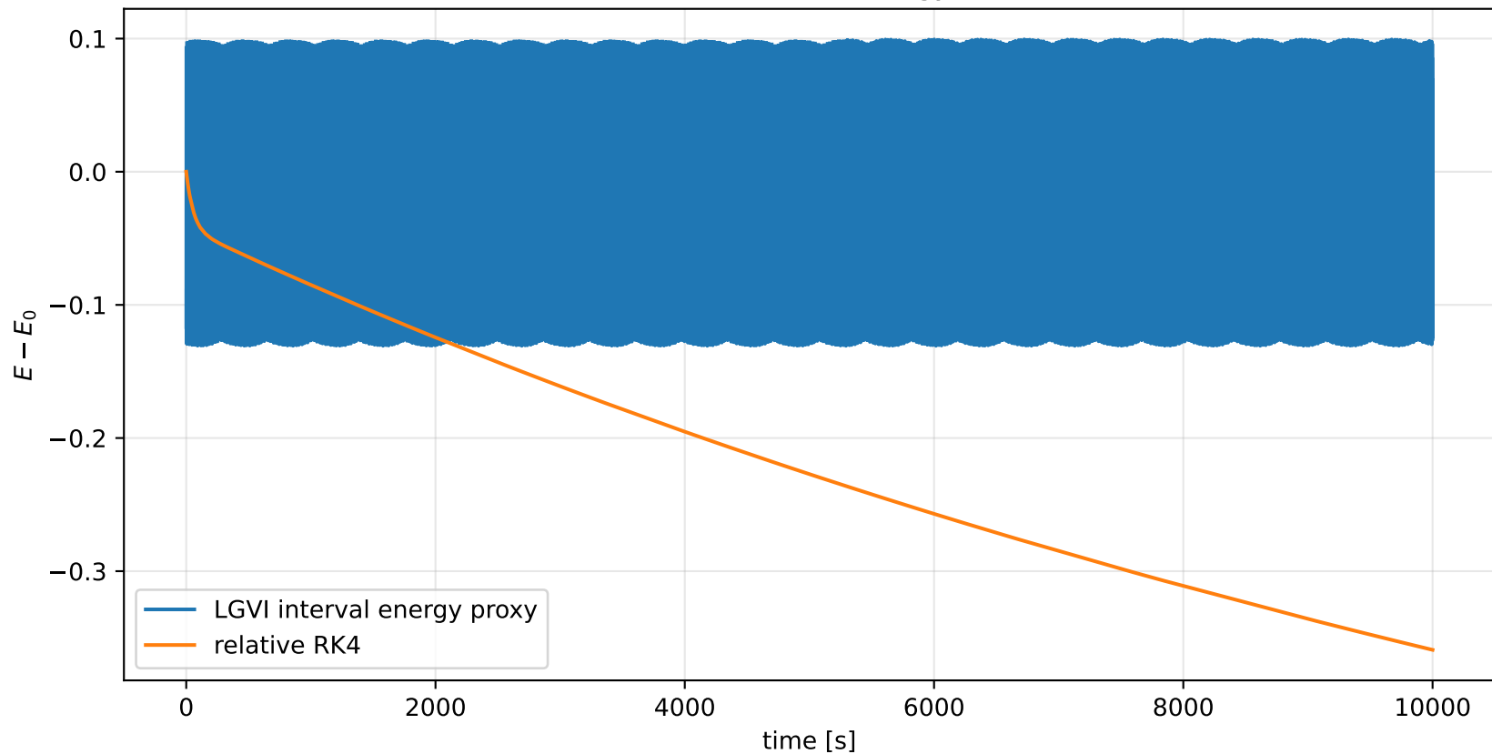
Unforced Acrobot energy error
