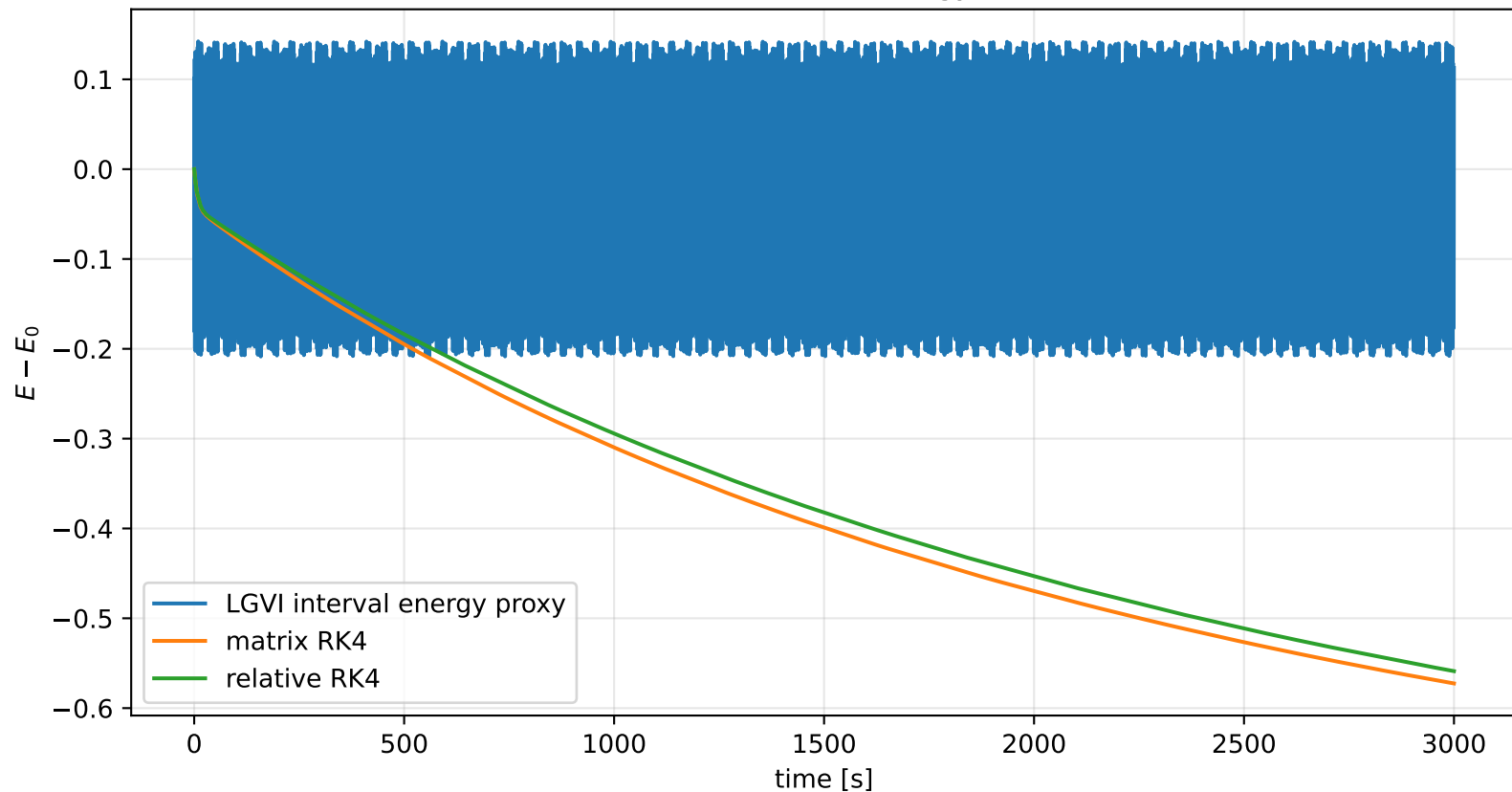
Unforced Acrobot energy error
