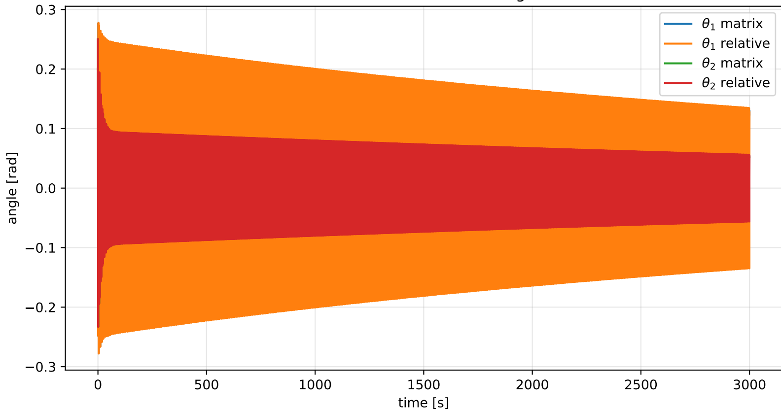
Continuous Acrobot RK4 angles
