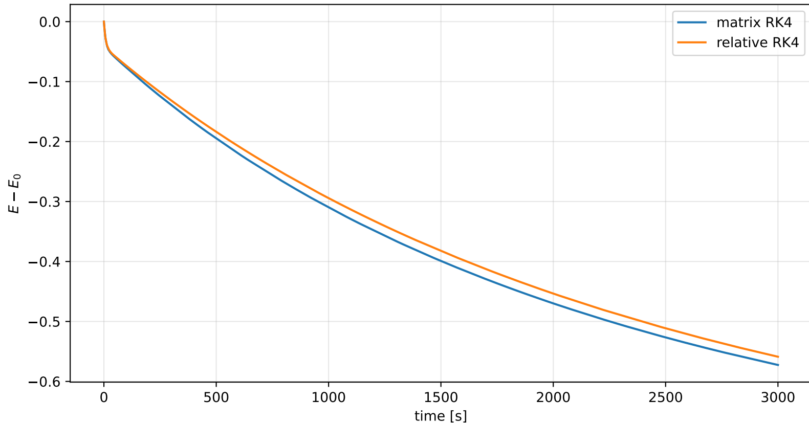
Unforced Acrobot RK4 energy error
