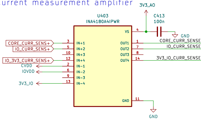
Current measurement amplifier
