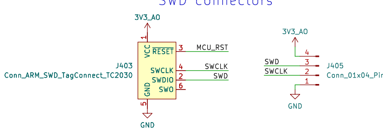
SWD connectors
