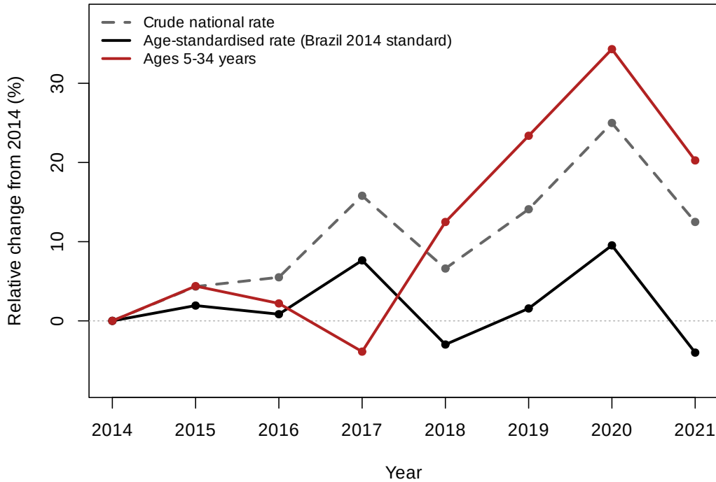
Figure 1: Relative change in each rate from its 2014 value, 2014–2021: crude national rate (dashed), age-standardised rate (Brazil 2014 standard, ages 7 or more) and rate at ages 5–34 years. Annual data; population from the IBGE 2018 projection.
