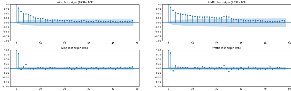
Fig. 7 ACF (top) and PACF (bottom) of the last evaluated h = 1 training window (720 observations) for wind (left) and traffic (right).
