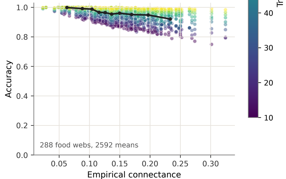
Accuracy
