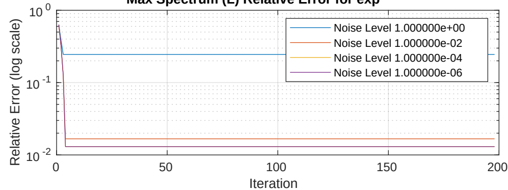
Max Spectrum (L) Relative Error for exp
