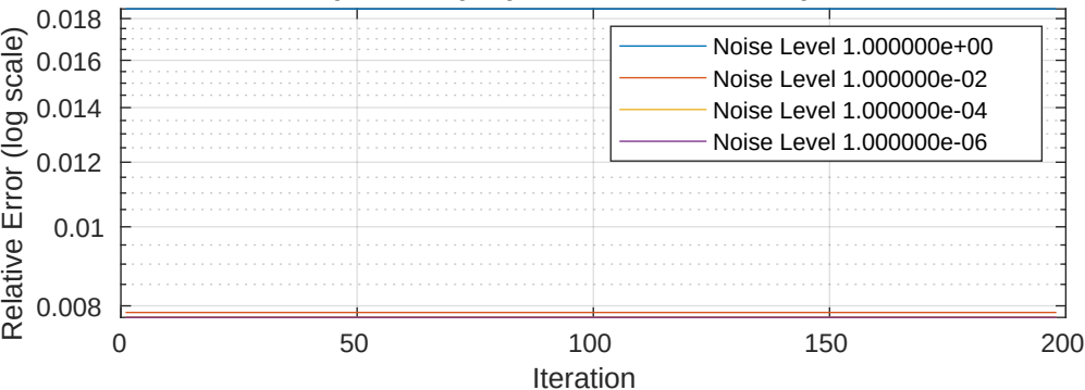
Max Spectrum (L) Relative Error for exp
