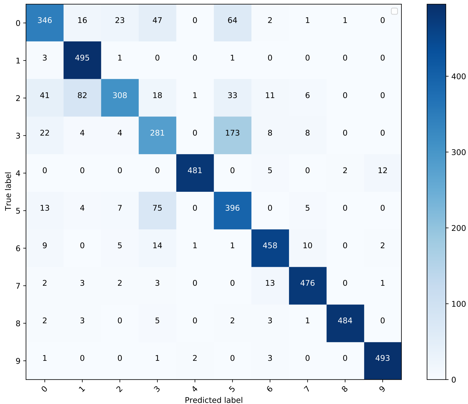
Confusion Matrix
