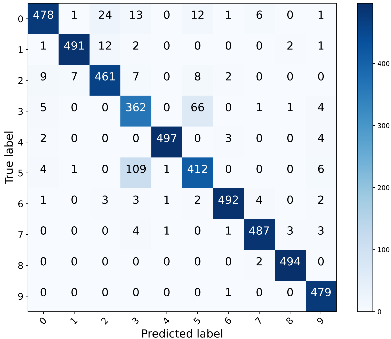
Confusion Matrix
