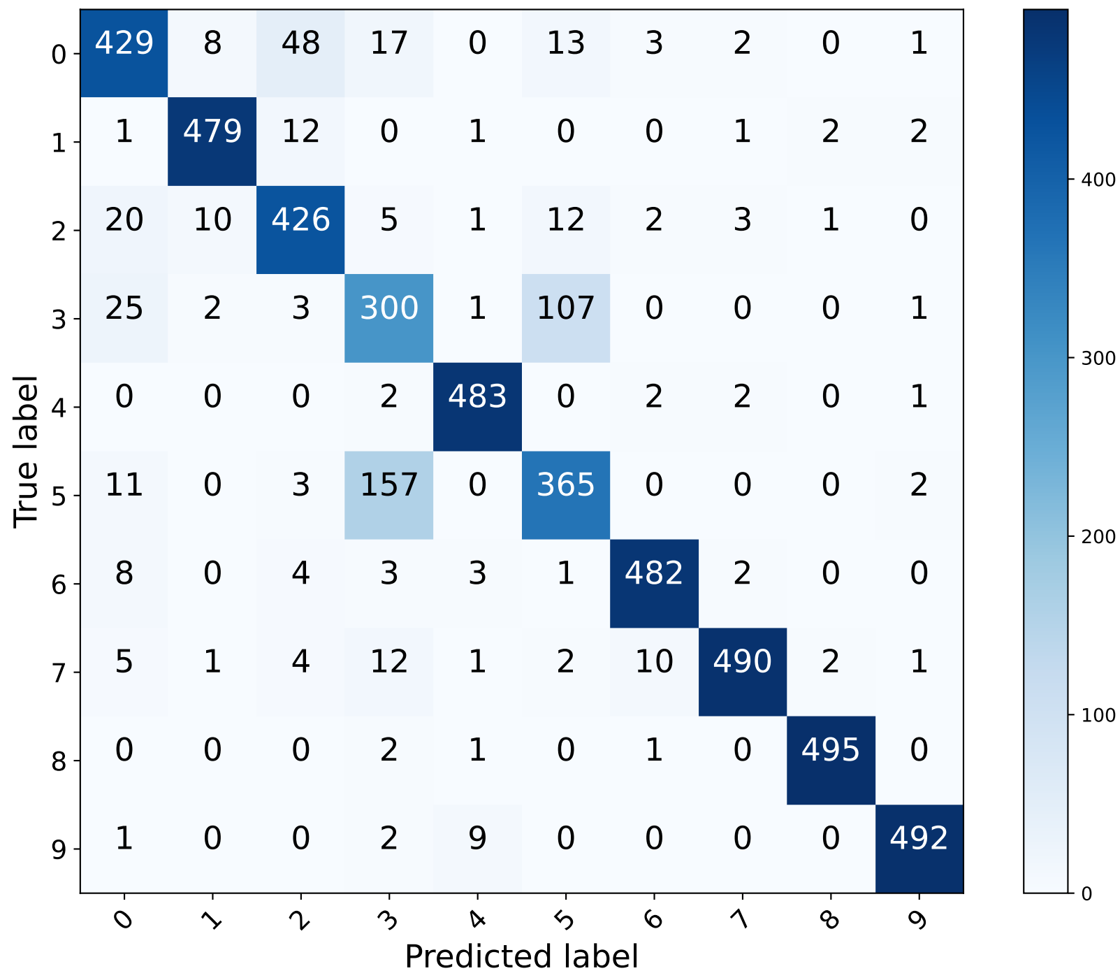
Confusion Matrix
