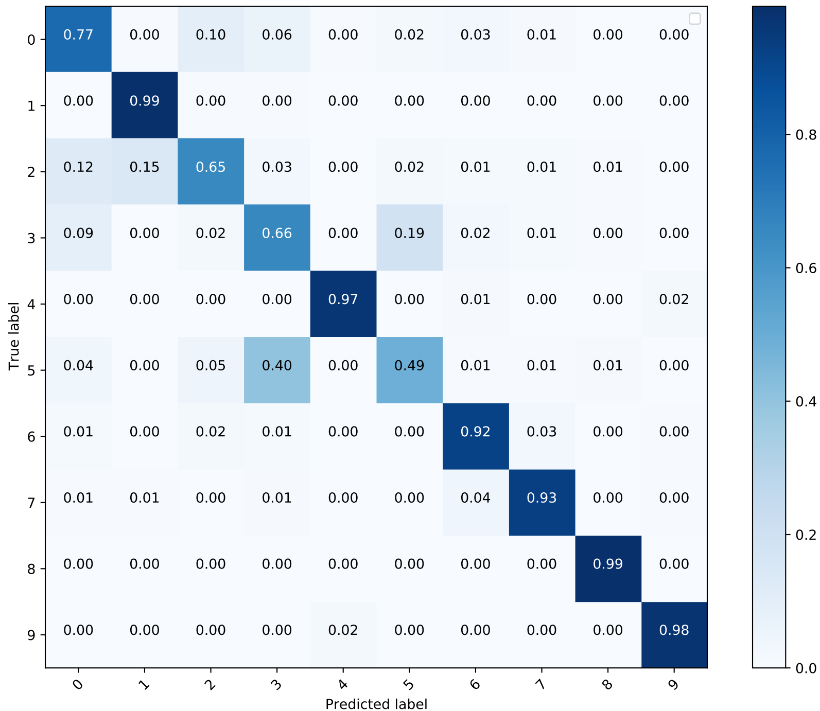
Normalized Confusion Matrix
