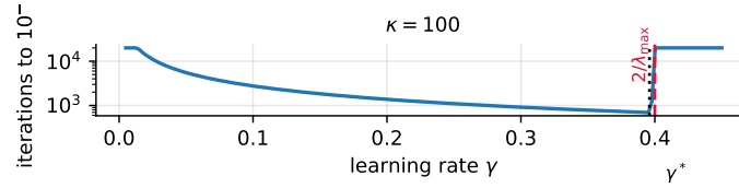
Fig. 4.1 Iterations required to reach an error of 10^{-6} against the learning rate, for a quadratic with eigenvalues \{0.05, 1, 5\} . The optimum lies at \gamma^* and the method diverges beyond 2/\lambda_{\max} , as predicted by Eqs. (4.20) and (4.21).
