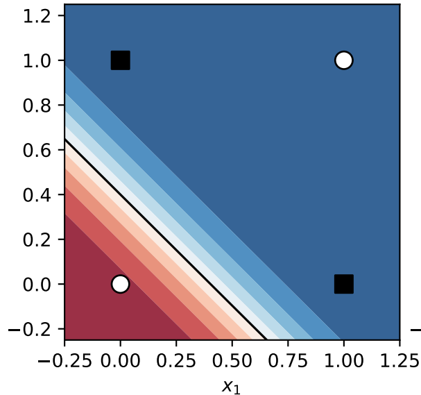
(a) hidden node 1: a_1^1 = \sigma(z_1^1)
