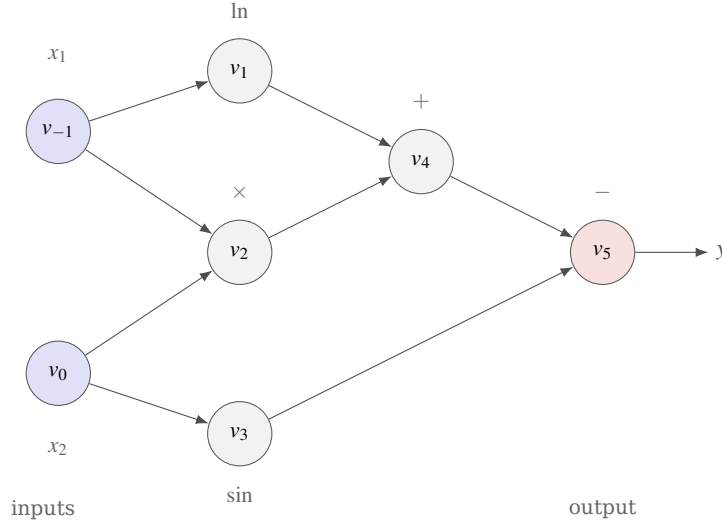
Fig. 4.5 The computational graph of the evaluation trace (4.53) for f(x_1, x_2) = \ln x_1 + x_1 x_2 - \sin x_2 . Each node is one elementary operation applied to its predecessors. Forward-mode AD sweeps this graph from left to right, carrying a derivative \dot{v}_i with every value; reverse-mode AD first evaluates the values from left to right and then sweeps back from right to left, carrying an adjoint \bar{v}_i = \partial y / \partial v_i with every node.
