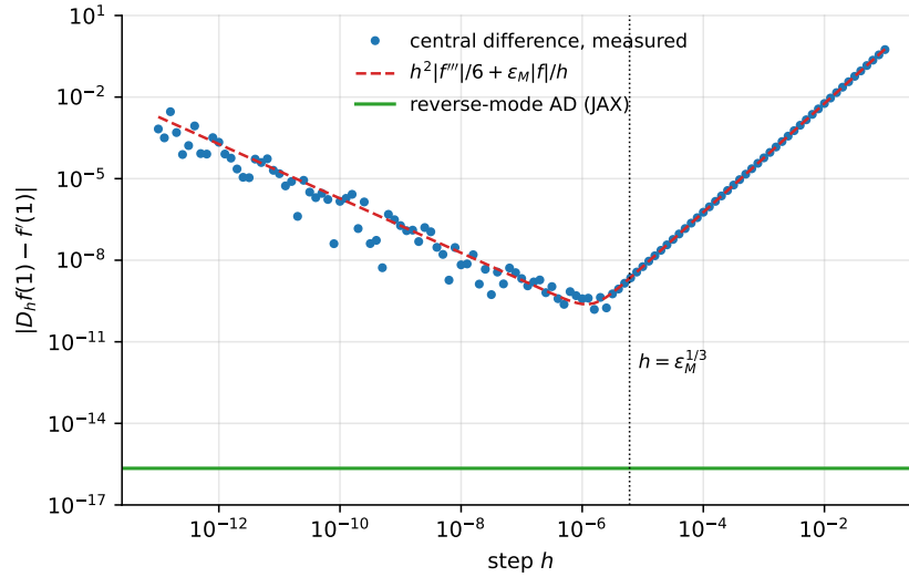
Fig. 4.6 Absolute error of the central finite difference (4.48) for f(x) = \sin(2\pi x + x^2) at x = 1 , as a function of the step h (points), together with the model (4.50) (dashed): truncation error \propto h^2 on the right, rounding error \propto 1/h on the left, and a minimum of about 10^{-10} near h \approx \epsilon_M^{1/3} . The reverse-mode derivative computed by JAX has an error at the level of the unit roundoff, shown as the horizontal line, for any h because it involves no h .
