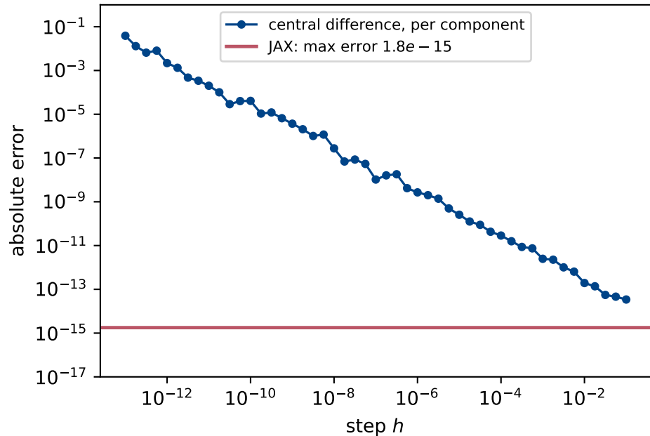
(b) the OLS gradient, degree 5: a quadratic cost
