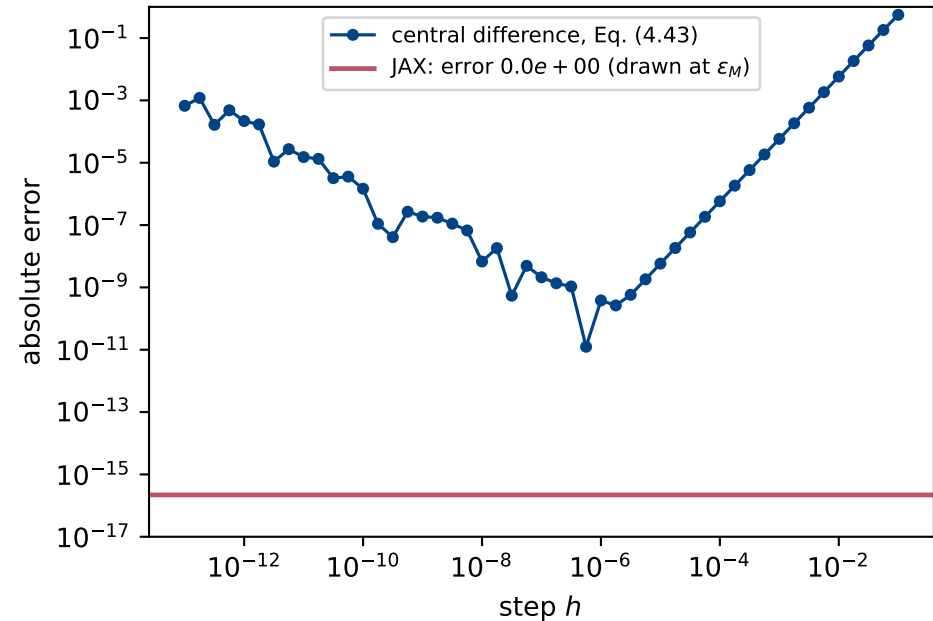
(a) f(x) = \sin(2\pi x + x^2) at x = 1 : h^2 truncation and 1/h rounding
