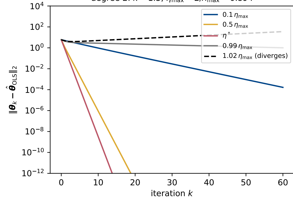
degree 2: \kappa = 1.3 , \eta_{\max} = 2/\lambda_{\max} = 0.894
