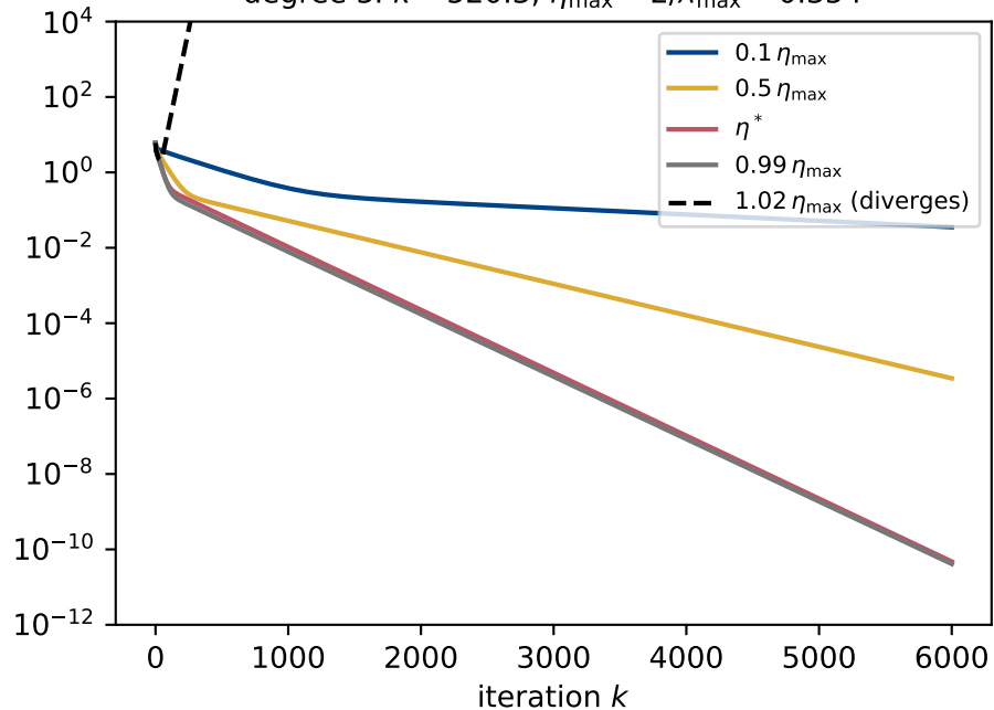
degree 5: \kappa = 520.3 , \eta_{\max} = 2/\lambda_{\max} = 0.354
