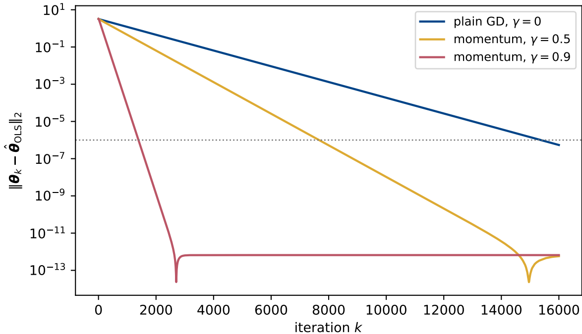
Runge function, degree 6: \kappa = 1849 , \eta = 0.9 \cdot 2/\lambda_{\max}
