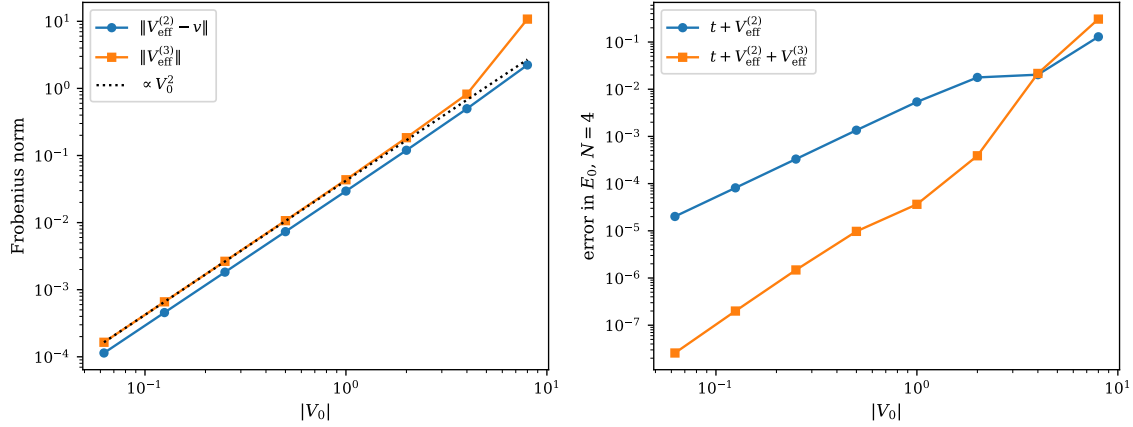
Fig. A.7 Left: Frobenius norms of the renormalisation of the two-body interaction, \|\hat{V}_{\text{eff}}^{(2)} - \hat{v}\| , and of the induced three-body interaction, \|\hat{V}_{\text{eff}}^{(3)}\| , as functions of the coupling |V_0| for n = 14 , n_p = 6 , \sigma = 1 and \Delta = 3 ; the dotted line is \propto V_0^2 . Right: the error in the four-particle ground-state energy of the model-space calculation with \hat{t} + \hat{V}_{\text{eff}}^{(2)} and with \hat{t} + \hat{V}_{\text{eff}}^{(2)} + \hat{V}_{\text{eff}}^{(3)} . Both norms follow the V_0^2 line at weak coupling; at V_0 = -4 the three-body term no longer improves the four-particle energy and at V_0 = -8 it makes it worse.
