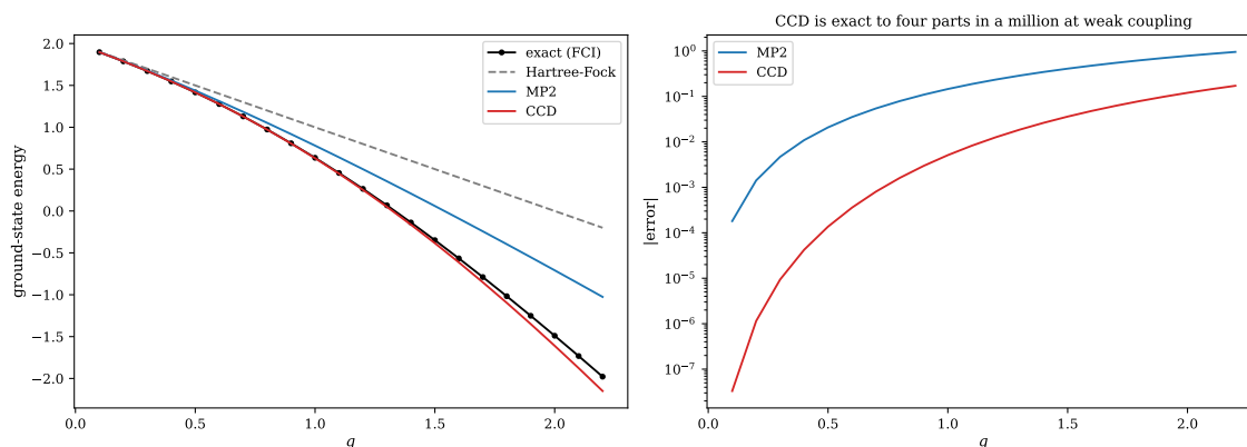
Fig. 10.2 Ground-state energy of the pairing model with four doubly degenerate levels, four particles and \xi = 1 , as a function of the pairing strength g over twenty-two values between 0.1 and 2.2. Left: the exact diagonalisation of Chapter 5 (black circles), the Hartree-Fock reference energy 2 - g (grey dashed), second-order Møller-Plesset theory (blue) and coupled-cluster doubles (red); the five couplings of Table 10.2 are points on these curves. Right: the absolute deviation of MP2 and of CCD from the exact energy on a logarithmic ordinate. The CCD curve lies three to four decades below the MP2 curve at weak coupling and the gap closes to less than one decade by g = 2.2 .
