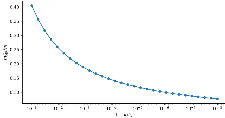
Fig. 6.10 Hartree-Fock effective mass (6.111) of the electron gas at r_s = 4 , in units of the bare mass, evaluated at thirty momenta approaching the Fermi surface from below and plotted against 1 - k/k_F on a logarithmic scale that runs from 10^{-1} on the left to 10^{-8} on the right, so that the Fermi surface lies at the right-hand edge. The ratio falls monotonically from 0.40 to 0.076, and it does so like the reciprocal of \ln(1 - k/k_F) : eight decades in the distance to the Fermi surface cost only a factor of five in m^* .
