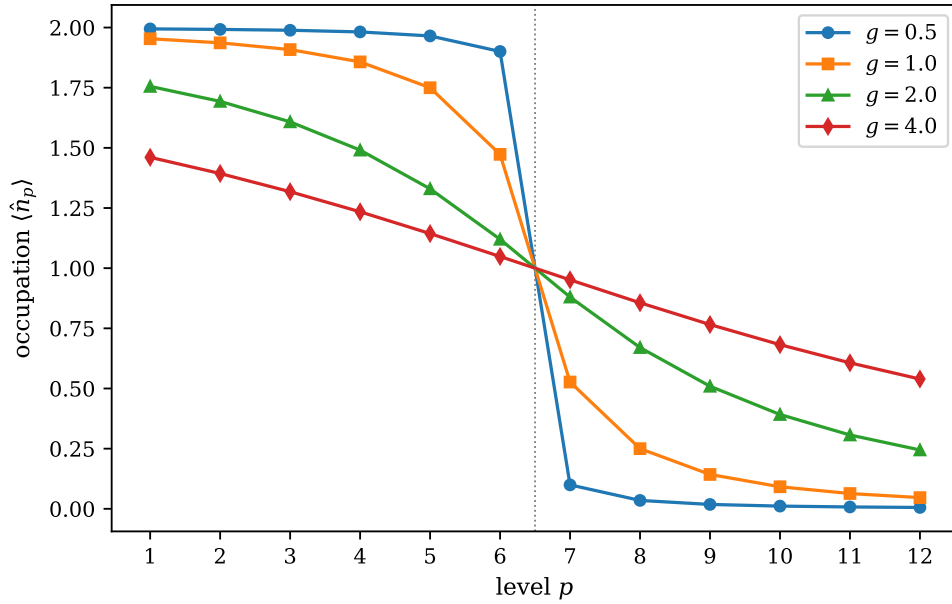
Fig. 11.2 Occupation numbers \langle \hat{n}_p \rangle of the twelve levels of the pairing model with six pairs from the DMRG ground state, for g = 0.5, 1, 2 and 4 . At weak coupling the Fermi surface between levels 6 and 7 is sharp; as g grows the pairs are scattered across it and the occupations are smeared, the correlated counterpart of the BCS smearing of Section 7.10, here without any breaking of particle-number conservation.
