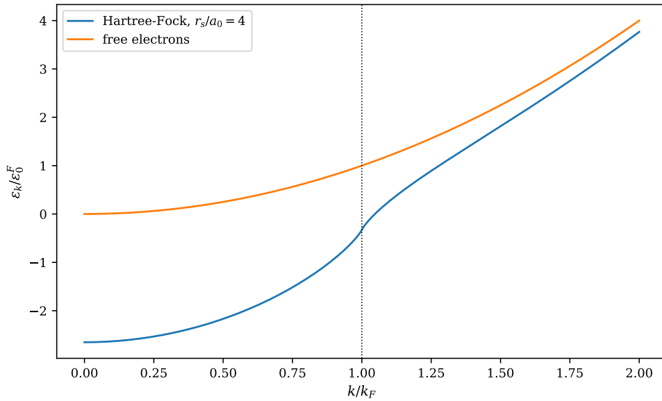
Fig. 6.9 Hartree-Fock single-particle energy of the three-dimensional electron gas, Eq. (6.107), at r_s = 4 , in units of the free Fermi energy \epsilon_0^F = \hbar^2 k_F^2 / 2m and against x = k/k_F , together with the free-particle parabola x^2 . The dotted vertical line marks the Fermi surface. Exchange lowers every level, by 2.652 at the bottom of the band and by only 1.326 at the Fermi surface, so the occupied band is stretched from a width of 1 to a width of 2.326; above k_F the two curves converge again as F(x) falls off, the gap being 0.233 at x = 2 .
