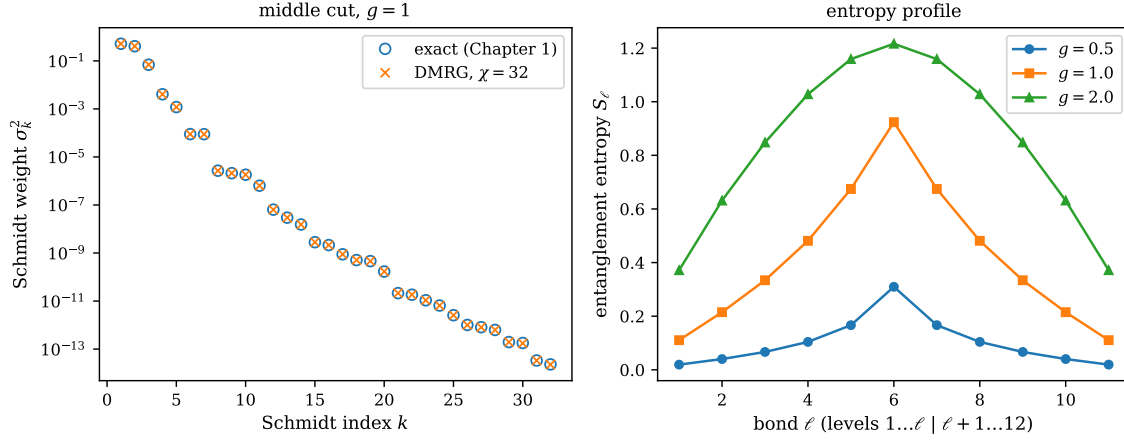
Fig. 11.1 The pairing model with twelve levels and six pairs, \xi = 1 . Left: the Schmidt weights \sigma_k^2 across the middle cut of the \chi = 32 DMRG state at g = 1 , against the exact weights of Fig. 1.6, which they reproduce to the last kept value. Right: the entanglement entropy across every bond of the chain for g = 0.5, 1 and 2 ; the bond \ell separates the lowest \ell levels from the rest, and the entropy is concentrated at the Fermi surface between levels 6 and 7.
