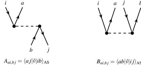
Fig. 6.8 The two blocks of the stability matrix, Eq. (6.78). Left: the particle-hole scattering diagram A , one pair in from below and one pair out above. Right: the pair-creation diagram B , two pairs out of the reference. With the excitation energies from the crosses, \Delta + A is the Tamm-Dancoff matrix and the full \hat{M} of Eq. (6.65) the matrix of the random-phase approximation.
