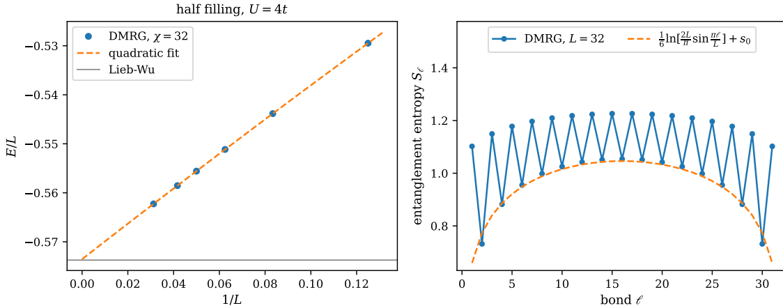
Fig. 11.4 The half-filled Hubbard chain with open ends at U = 4t . Left: the DMRG energy per site against 1/L for L = 8 to 32 at \chi = 32 ; the dashed curve is the quadratic fit in 1/L and the horizontal line the Bethe-ansatz energy of the infinite chain, Eq. (11.11). Right: the entanglement entropy across every bond \ell of the L = 32 chain, with the conformal prediction S_\ell = \frac{c}{6} \ln \left[ \frac{2L}{\pi} \sin \frac{\pi \ell}{L} \right] + s_0 for c = 1 drawn through the even bonds.
