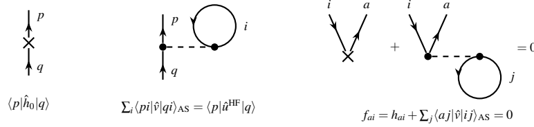
Fig. 6.6 Left and middle: the two open diagrams with one line in and one line out, the bare one-body vertex and the bubble insertion. Their sum is the Fock matrix f_{pq} , Eq. (6.76); the bubble insertion alone is the Hartree-Fock potential \hat{u}^{\text{HF}} . Right: the Hartree-Fock condition, Eq. (6.77) – the same two diagrams with the line in taken as a hole i and the line out as a particle a , required to add up to zero.
