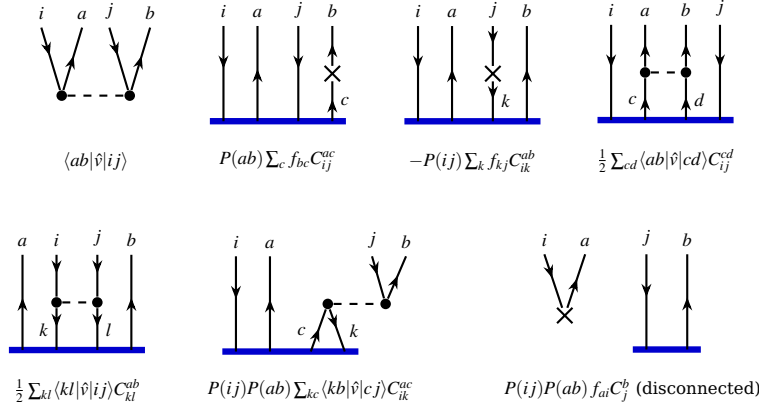
Fig. 5.7 Diagrams of the doubles equation, Eq. (5.49), with the open lines a, b and i, j of the bra \langle\Phi_{ij}^{ab}| . Top row and first two of the bottom row: the driving term and the five doubles-doubles terms of the first line of the equation – the crosses on an open line, the particle-particle and hole-hole ladders, and the ring. Bottom right: the disconnected singles term P(ij)P(ab)f_{ai}C_j^b , two pieces sharing no line.
