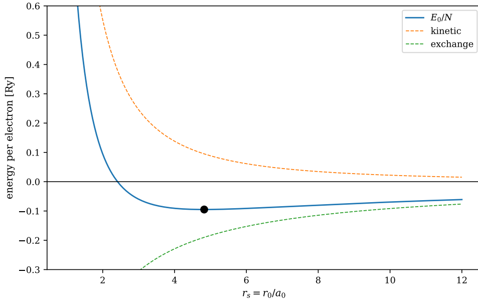
Fig. 6.11 Hartree-Fock energy per electron of the three-dimensional electron gas, Eq. (6.113), in Rydberg and against the density parameter r_s = r_0/a_0 , decomposed into the kinetic term 2.21/r_s^2 and the exchange term -0.916/r_s . The two contributions carry opposite signs and different powers of the density, so their sum turns over; the filled circle marks the minimum at r_s = 4.83 , where E_0/N = -0.0949 Ry = -1.29 eV. The total crosses zero at r_s = 2.41 and the well is very shallow, the energy staying within 5% of its minimum over the whole interval 4 \leq r_s \leq 6 .
