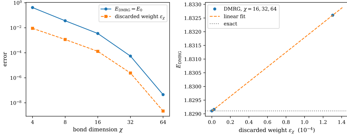
Fig. 11.3 Convergence of the DMRG for the pairing plus particle-hole model, eight levels, eight particles, g = 1 , f = 0.5 . Left: the energy error against the bond dimension, on a logarithmic scale. Right: the energy against the largest discarded weight of the final sweep for \chi = 16, 32 and 64 ; the dashed line is a straight-line fit through the three points, and its intercept at \epsilon_\chi = 0 is the extrapolated energy. The dotted horizontal line is the exact energy.
