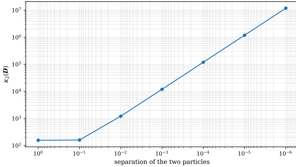
Fig. 2.4 Condition number \kappa_2(\mathbf{D}) = \sigma_0/\sigma_{N-1} of the Slater matrix for six particles in a two-dimensional oscillator basis, as two of the six are brought together while the other four are held fixed. Both axes are logarithmic and the abscissa is reversed, so that the approach to the nodal surface runs from left to right. For separations above about 0.1 oscillator lengths the condition number is flat at \kappa_2 \simeq 1.5 \times 10^2 , a value set by the shape of the basis and by the random placement of the spectator particles; below that it rises by exactly one decade for every decade of approach, reaching 1.2 \times 10^7 at a separation of 10^{-6} . The straight line of unit slope is the signature of a simple zero of |\mathbf{D}| on the nodal surface.
