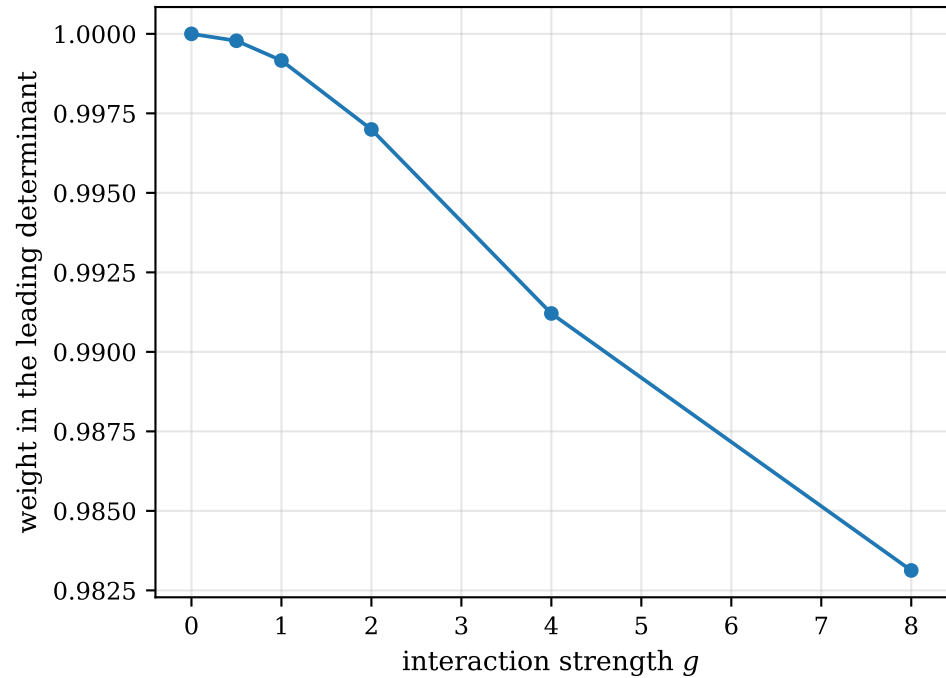
Departure from a single determinant
