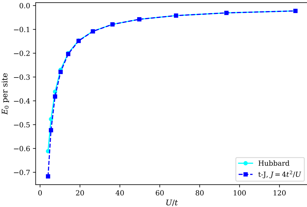
half-filled 6-site ring
