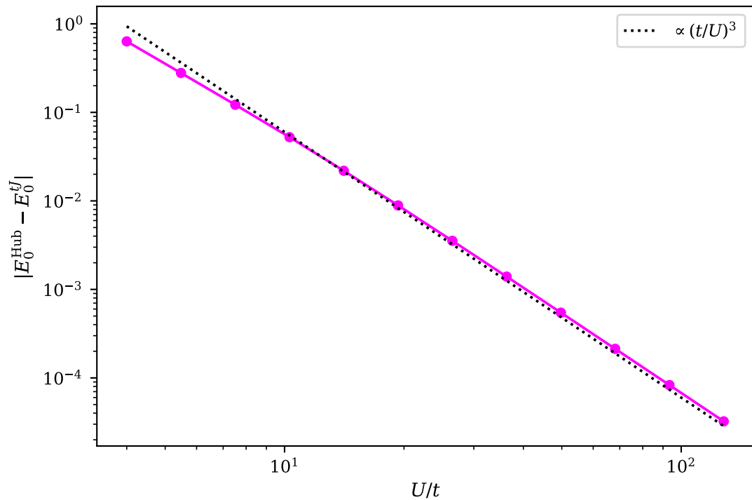
truncated ring-exchange terms
