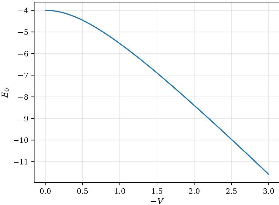
Lipkin ground-state energy
