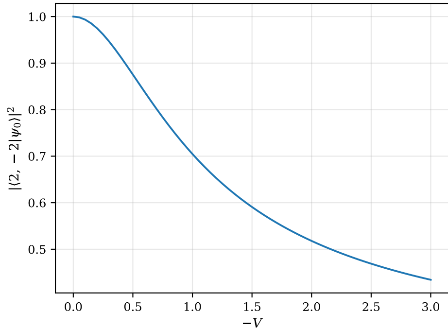
Weight of the unperturbed configuration
