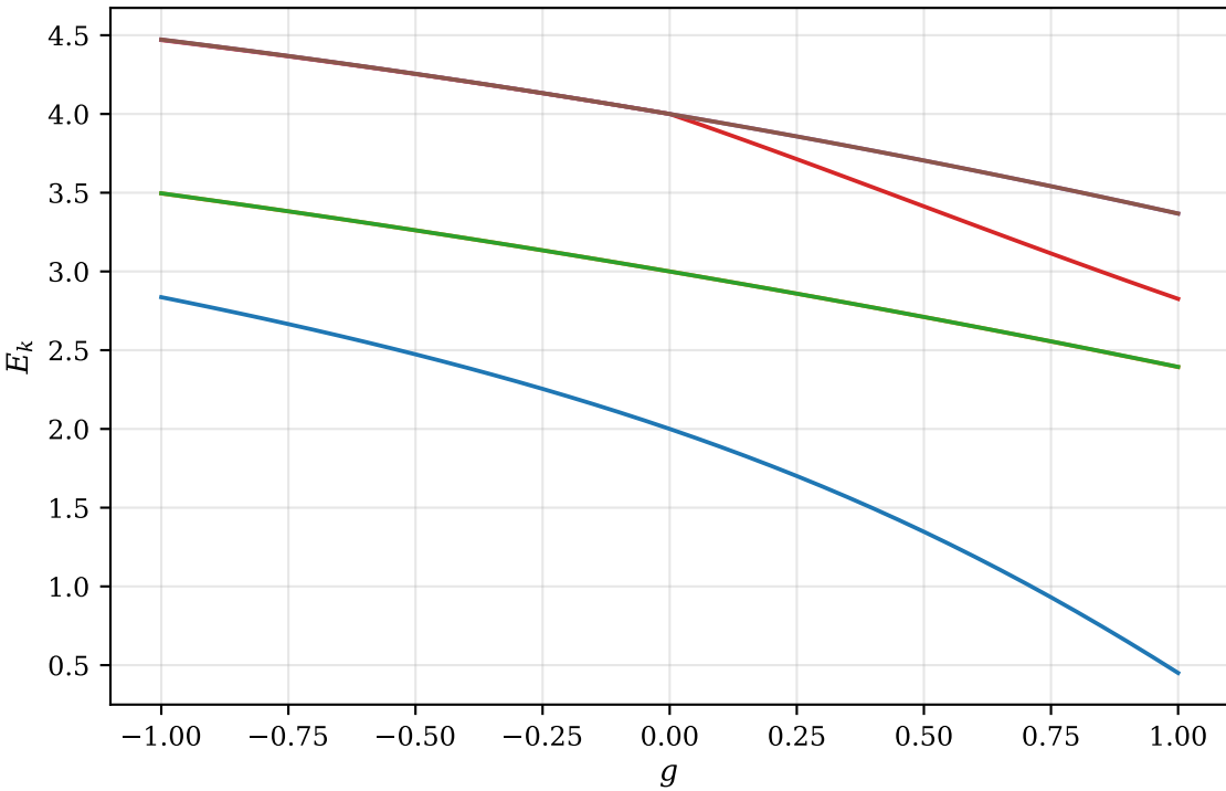
exact eigenvalues, f = 0.05 g
