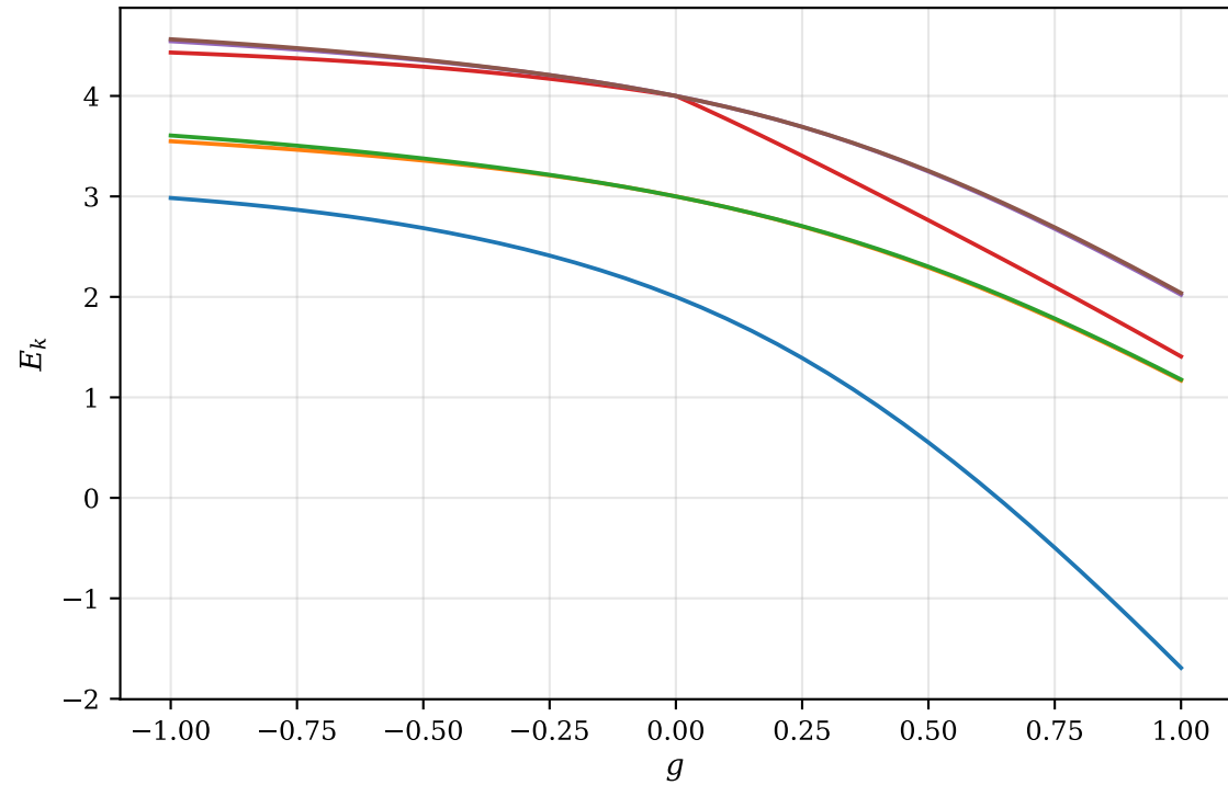
exact eigenvalues, f = 0.5 g
