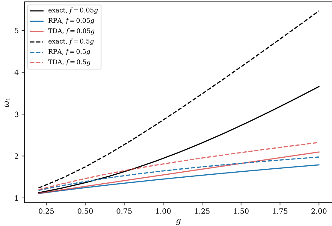
lowest excitation
