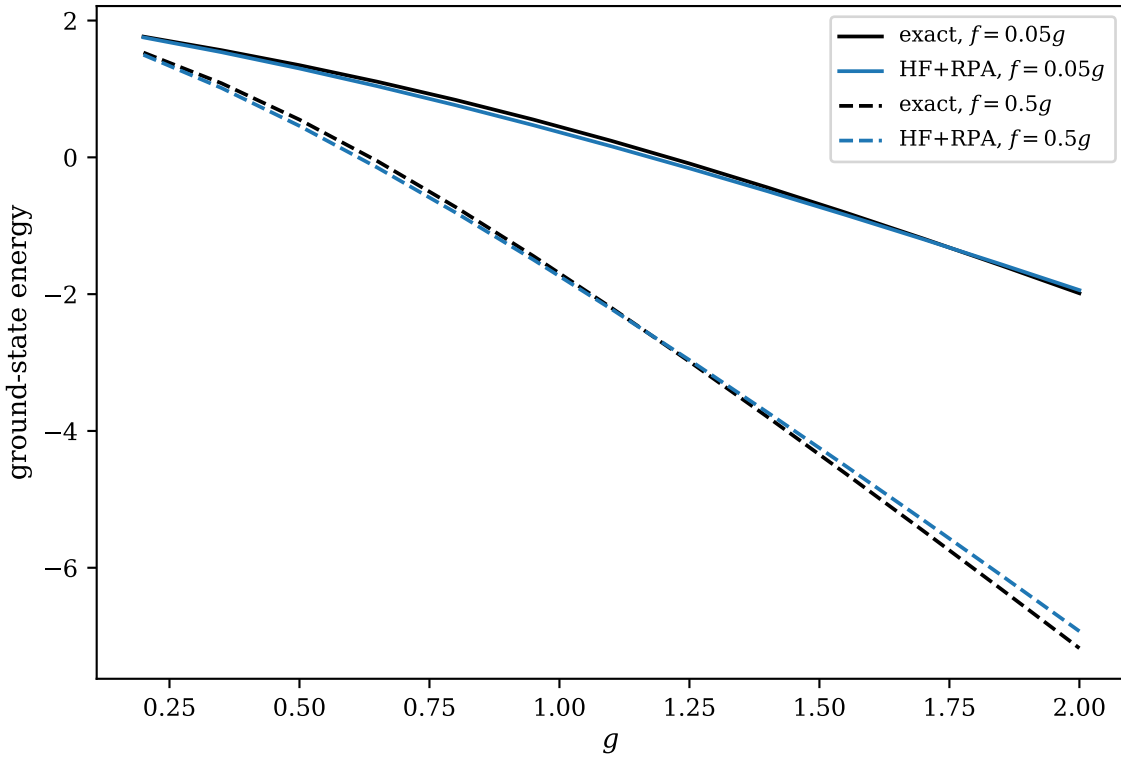
ground state
