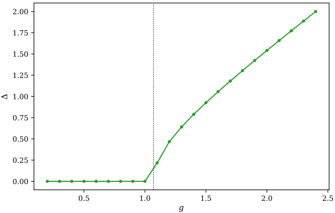
pairing gap; g_c = 1.07037
