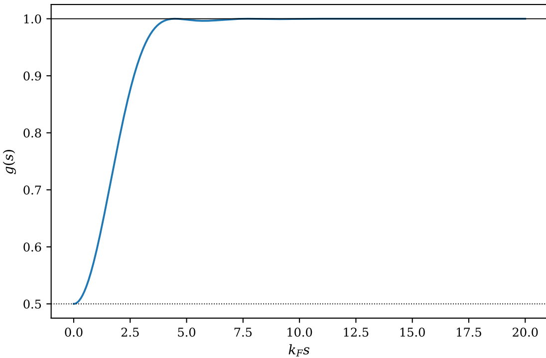
pair correlation function
