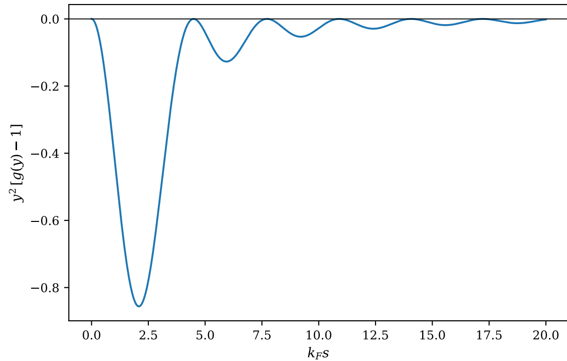
the sum-rule integrand
