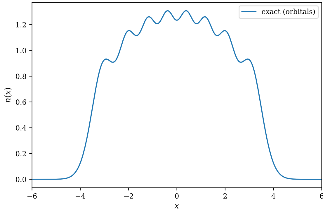
the shell structure Thomas-Fermi cannot produce
