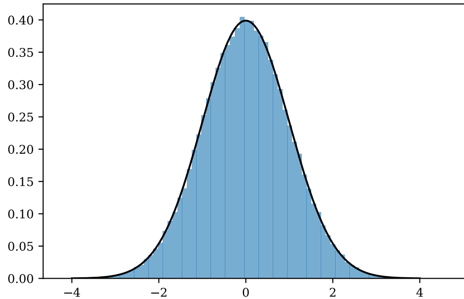
Box-Muller normal
