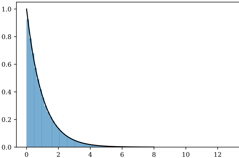
exponential
