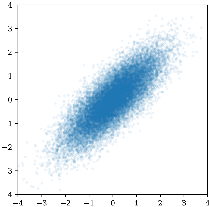
direct draws
