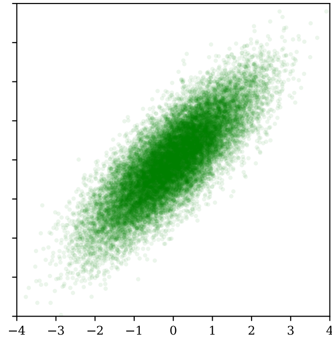
Gibbs samples
