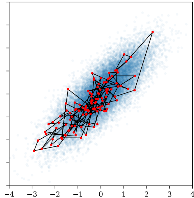
the Gibbs path (120 sweeps)
