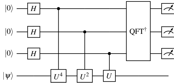
Fig. 19.3 Quantum phase estimation with a three-qubit control register. Hadamards, then controlled powers U^{2^j} , then the inverse QFT, then measurement. The system register emerges in the state it entered.
