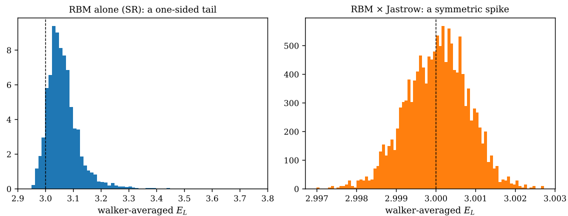
Fig. A.19 Distribution of the walker-averaged local energy in the production run of the four-unit machine trained by stochastic reconfiguration, without (left) and with (right) the Padé-Jastrow factor. The dashed line is the exact energy 3. Note the different horizontal scales: the left panel has the one-sided tail of an ansatz without a cusp, the right one is a symmetric spike a few thousandths wide.
