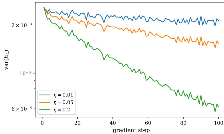
Fig. A.16 One particle in one dimension without interaction, two hidden units: the variance of the local energy during a hundred steps of gradient descent for three learning rates. The exact ground state has zero variance and is representable exactly, so the variance measures the distance from the solution.
