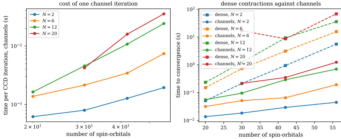
Fig. A.13 Cost of the CCD solvers against the size of the basis, for N = 2, 6, 12 and 20 electrons at \omega = 1 . Left: the time of one iteration of the channel code. Right: the time to convergence of the dense solver of Chapter 10 (dashed) and of the channel code (solid), on a logarithmic scale. The dense solver at 30 orbitals and N = 20 is slow because only ten virtual orbitals are available and the iteration converges poorly.
