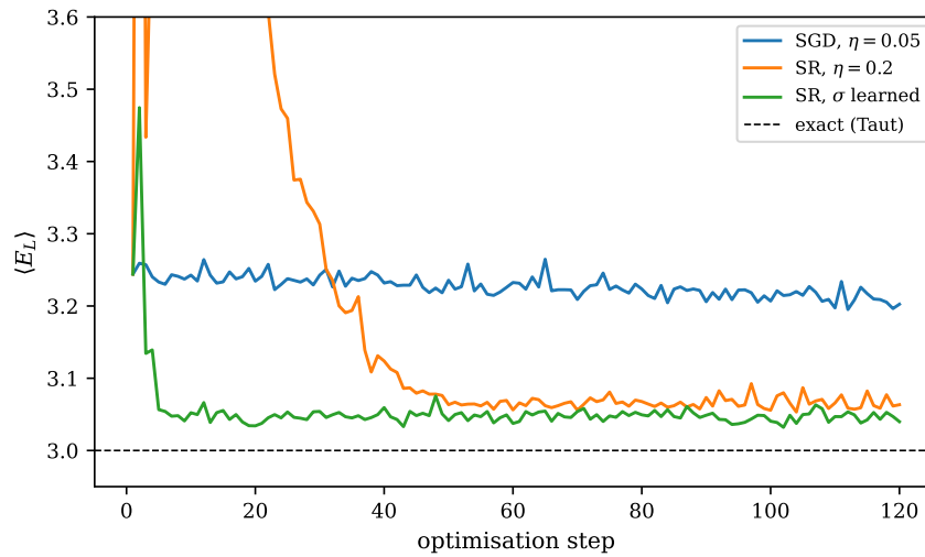
Fig. A.18 The interacting dot with four hidden units: the Monte Carlo estimate of the energy at each optimisation step for gradient descent at \eta = 0.05 , stochastic reconfiguration at \eta = 0.2 , and stochastic reconfiguration with the width \sigma as a variational parameter, all from the same start. The dashed line is Taut's exact energy.
