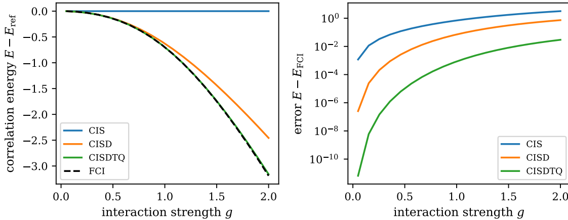
Fig. 5.2 Truncated configuration interaction against full CI for the pairing Hamiltonian of Eq. (5.34) with six doubly degenerate levels, six particles and \xi = 1 , over the range 0.05 \leq g \leq 2 . The left panel shows the correlation energy E - E_{\text{ref}} recovered by CIS, CISD and CISDTQ, together with the full CI result as a dashed line; the right panel shows what each truncation misses, E - E_{\text{FCI}} , on a logarithmic scale. The full space holds \binom{12}{6} = 924 determinants, with excitations up to 6p-6h , and the truncated spaces 37, 262 and 887 of them, so that the quadruples are a genuine truncation and not the whole space in disguise. The errors climb by six to ten orders of magnitude across the range while the truncation level stays fixed.
