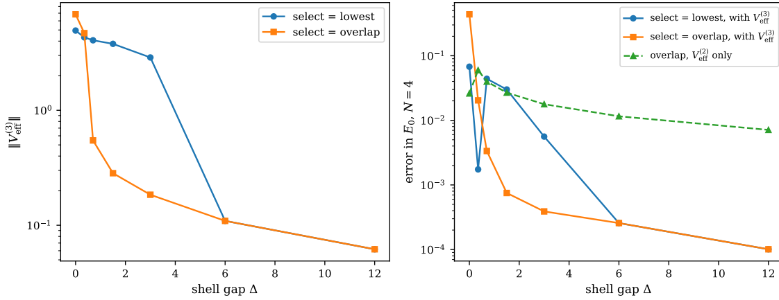
Fig. A.9 The intruder-state problem. Left: the norm of the induced three-body interaction as a function of the shell gap \Delta , for the two rules of Table A.2 (lowest and overlap in the program). Right: the error of the four-particle ground state with \hat{t} + \hat{V}_{\text{eff}}^{(2)} + \hat{V}_{\text{eff}}^{(3)} for both rules, and with \hat{t} + \hat{V}_{\text{eff}}^{(2)} alone for the largest-norm rule. Below \Delta \approx 5 the lowest-eigenvalue rule picks up intruders; the largest-norm rule survives to \Delta \approx 0.7 and fails at the pure oscillator, \Delta = 0 .
