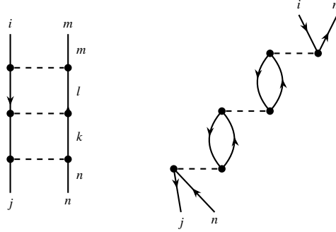
Fig. 7.7 The Tamm-Dancoff approximation sums all forward-going scatterings of one particle-hole pair. Left: the exchange part of the antisymmetrised vertex, a particle-hole ladder. Right: the direct part, a chain of bubbles in which the pair annihilates on one vertex and a new pair is created on the other. Both are the same term \bar{v}_{mjn} of A applied repeatedly; the crosses supplying \epsilon_m - \epsilon_i on each segment are not drawn.
