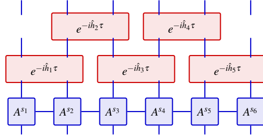
Fig. 11.8 One first-order Trotter step on a chain of six sites: a layer of gates on the odd bonds followed by a layer on the even bonds, each gate a d^2 \times d^2 unitary acting on two physical legs. Each gate is an MPO of two sites and bond dimension at most d^2 , Eq. (11.39), so a layer is an MPO whose bond dimension alternates between d^2 and one.
