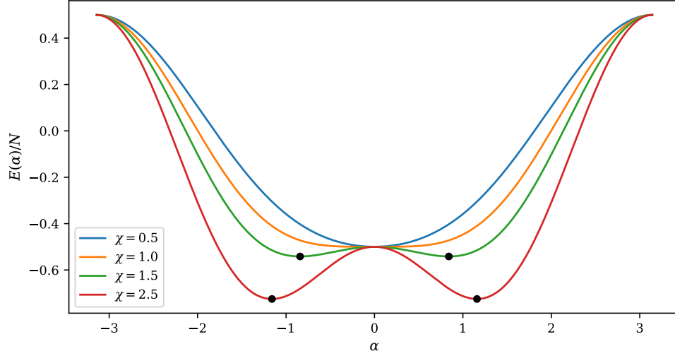
Fig. 6.3 The Lipkin mean-field energy per particle E(\alpha)/N of Eq. (6.90) against the Thouless rotation angle \alpha , for N = 4 , \varepsilon = 1 , W = 0 and four values of the dimensionless coupling \chi = |V|(N-1)/\varepsilon . All four curves pass through E/N = -\varepsilon/2 at \alpha = 0 , the spherical solution. For \chi < 1 that point is the global minimum; at \chi = 1 the curvature vanishes and the surface is quartic there; for \chi > 1 it has become a local maximum and two degenerate deformed minima, marked by the filled circles, have moved out to \cos \alpha = 1/\chi .
