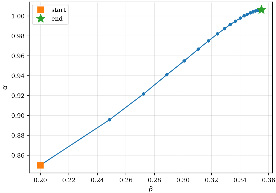
Fig. 15.1 The descent of Table 15.2 drawn as a path in the plane of the two variational parameters, with \beta horizontal and \alpha vertical, over twenty steps of Eq. (15.19) at a fixed learning rate \eta = 0.05 . The square marks the deliberately poor starting point (\alpha, \beta) = (0.85, 0.20) , the star the point (1.0062, 0.3553) reached after twenty steps, and the circles between them the individual iterates, each obtained from its own short Monte Carlo run. Since the step is -\eta \nabla E , the spacing of the circles is a direct picture of the length of the gradient, which falls from 1.32 at the start to 0.028 at the end.
