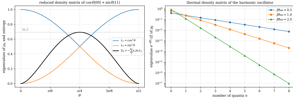
Fig. 1.2 Two readings of the spectrum of a density matrix. Left: the eigenvalues \{\cos^2\theta, \sin^2\theta\} of the reduced density matrix \rho_A of the two-qubit state \cos\theta|00\rangle + \sin\theta|11\rangle and the entanglement entropy of Eq. (1.6), which rises from 0 at the product state to \ln 2 at the Bell state. Right: the eigenvalues of the thermal density matrix (1.4) of the harmonic oscillator, which are the Boltzmann weights e^{-\beta E_n}/Z of the number states, for three temperatures.
