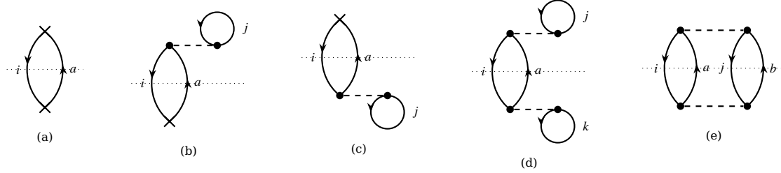
Fig. 9.6 The five second-order diagrams, Eq. (9.42). The dotted line is the cut whose crossing lines determine the denominator. (a) Two crosses; (b), (c) a cross and a bubble insertion in the two time orderings; (d) two bubble insertions; (e) two pairs created and annihilated, the second-order ring. Diagrams (a)–(d) go through single excitations and add up to \sum_{ai} |f_{ai}|^2 / (\epsilon_i - \epsilon_a) ; diagram (e) goes through double excitations and is the Møller-Plesset second-order energy (9.30).
