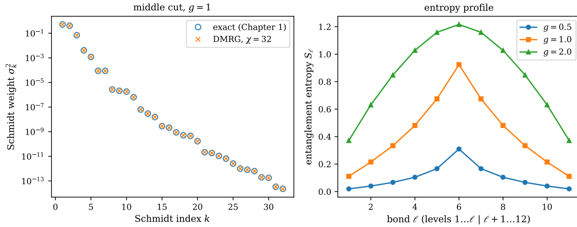
Fig. 11.4 The pairing model with twelve levels and six pairs, \xi = 1 . Left: the Schmidt weights \sigma_k^2 across the middle cut of the \chi = 32 DMRG state at g = 1 , against the exact weights of Fig. 1.6, which they reproduce to the last kept value. Right: the entanglement entropy across every bond of the chain for g = 0.5, 1 and 2 ; the bond \ell separates the lowest \ell levels from the rest, and the entropy is concentrated at the Fermi surface between levels 6 and 7.
