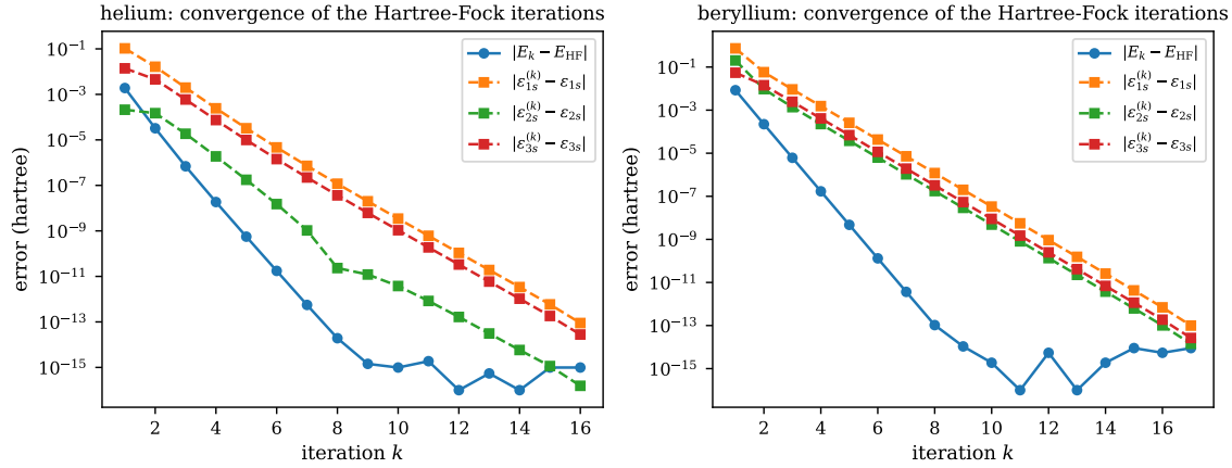
Fig. A.10 Convergence of the Hartree-Fock iterations for helium (left) and beryllium (right) in the hydrogenic 1s-2s-3s basis: the error of the total energy and of the three orbital energies against the iteration number, on a logarithmic scale. The energy, which is stationary at the solution, converges at twice the rate of the orbital energies.
