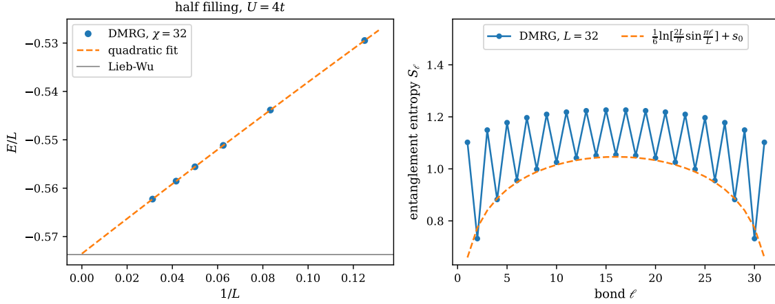
Fig. 11.7 The half-filled Hubbard chain with open ends at U = 4t . Left: the DMRG energy per site against 1/L for L = 8 to 32 at \chi = 32 ; the dashed curve is the quadratic fit in 1/L and the horizontal line the Bethe-ansatz energy of the infinite chain, Eq. (11.37). Right: the entanglement entropy across every bond \ell of the L = 32 chain, with the conformal prediction S_\ell = \frac{c}{6} \ln \left[ \frac{2L}{\pi} \sin \frac{\pi \ell}{L} \right] + s_0 for c = 1 drawn through the even bonds.
