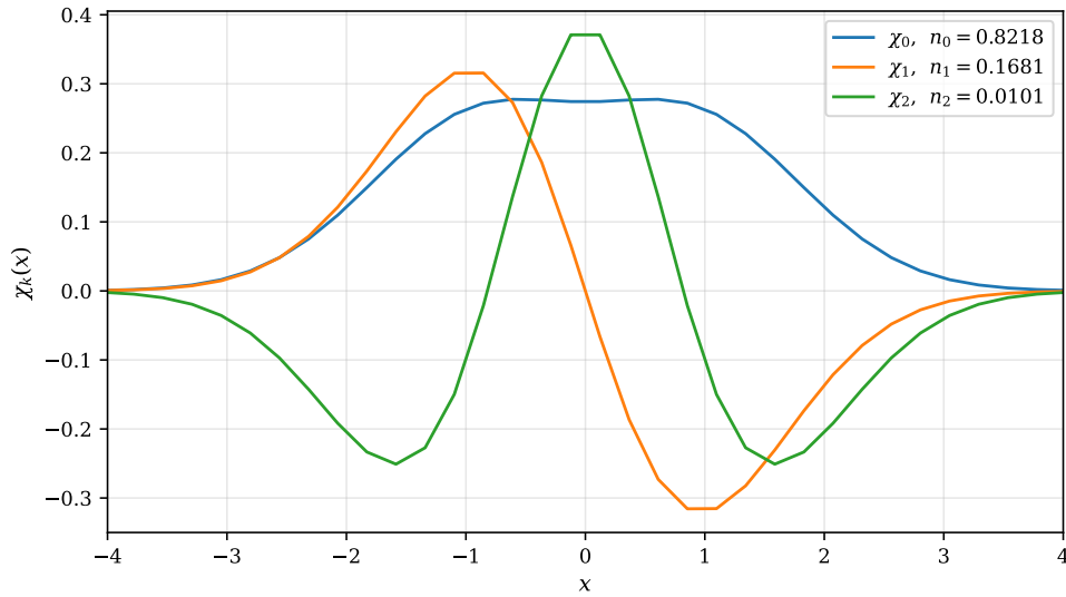
Fig. 1.7 The three leading natural orbitals \chi_k(x) of two particles in a one-dimensional harmonic trap with a softened Coulomb repulsion of strength g = 5 , obtained as the eigenvectors of the one-body density matrix (1.118) on a grid of 40 points. The legend gives the corresponding occupation numbers. The leading orbital carries n_0 = 0.8218 and is nodeless but visibly flattened at the centre; the second, with n_1 = 0.1681 , is odd with one node; the third, with n_2 = 0.0101 , is even with two. The orbitals are ordered by occupation, not by energy, and the sign of each is fixed by requiring its largest component to be positive.
