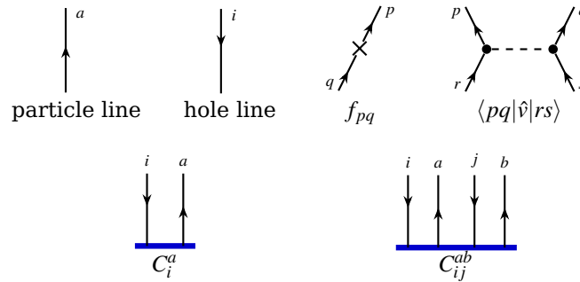
Fig. 5.4 The elements of the diagrams for the full CI equations. Time runs upward and the reference determinant is not drawn. Top row: a particle line (arrow up), a hole line (arrow down), the one-body vertex of \hat{F}_N with the element f_{pq} ( p out, q in), and the two-body interaction \hat{V}_N with the element \langle pq | \hat{v} | rs \rangle , one index pair per vertex. Bottom row: the amplitude bars C_1 and C_2 , from which one and two particle-hole pairs emerge; C_3 has three, and so on.
