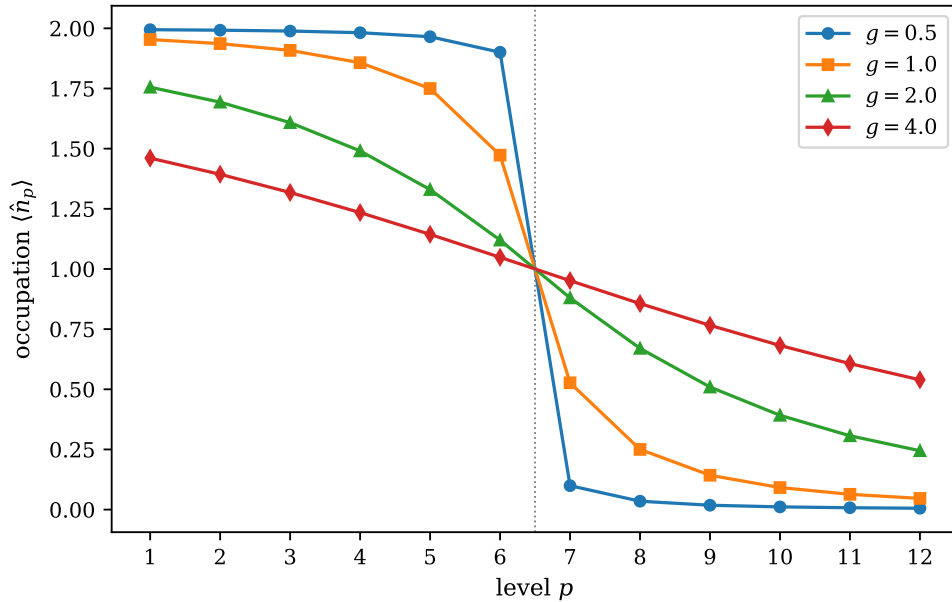
Fig. 11.5 Occupation numbers \langle \hat{n}_p \rangle of the twelve levels of the pairing model with six pairs from the DMRG ground state, for g = 0.5, 1, 2 and 4 . At weak coupling the Fermi surface between levels 6 and 7 is sharp; as g grows the pairs are scattered across it and the occupations are smeared, the correlated counterpart of the BCS smearing of Section 7.10, here without any breaking of particle-number conservation.
