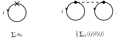
Fig. 9.4 The two first-order diagrams, Eq. (9.40): the one-body remainder closed by a bubble, and the interaction with a bubble on each vertex. Together they are E_{\text{ref}} - W_0 .
