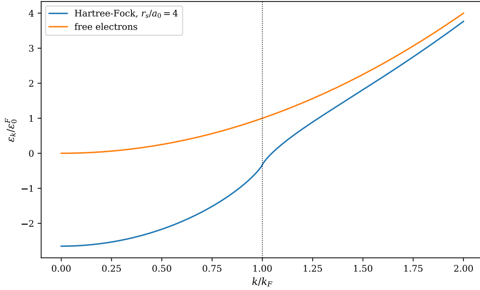
Fig. 6.9 Hartree-Fock single-particle energy of the three-dimensional electron gas, Eq. (6.127), at r_s = 4 , in units of the free Fermi energy \varepsilon_0^F = \hbar^2 k_F^2 / 2m and against x = k/k_F , together with the free-particle parabola x^2 . The dotted vertical line marks the Fermi surface. Exchange lowers every level, by 2.652 at the bottom of the band and by only 1.326 at the Fermi surface, so the occupied band is stretched from a width of 1 to a width of 2.326; above k_F the two curves converge again as F(x) falls off, the gap being 0.233 at x = 2 .
