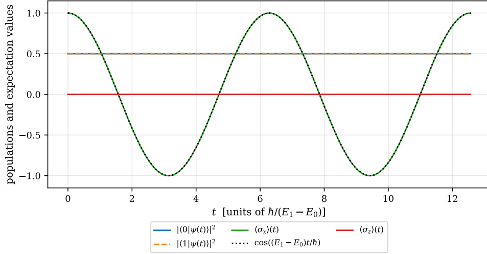
Fig. 1.1 Time evolution of the two-level state (|0\rangle + |1\rangle)/\sqrt{2} under \mathbf{H} = E_0|0\rangle\langle 0| + E_1|1\rangle\langle 1| , computed from Eq. (1.5) with E_1 - E_0 = 1 and \hbar = 1 . The populations |\langle 0|\psi(t)\rangle|^2 and |\langle 1|\psi(t)\rangle|^2 are constant, since each energy component only acquires a phase; \langle \sigma_x \rangle oscillates at the Bohr frequency because the relative phase e^{-i(E_1 - E_0)t/\hbar} rotates the state.
