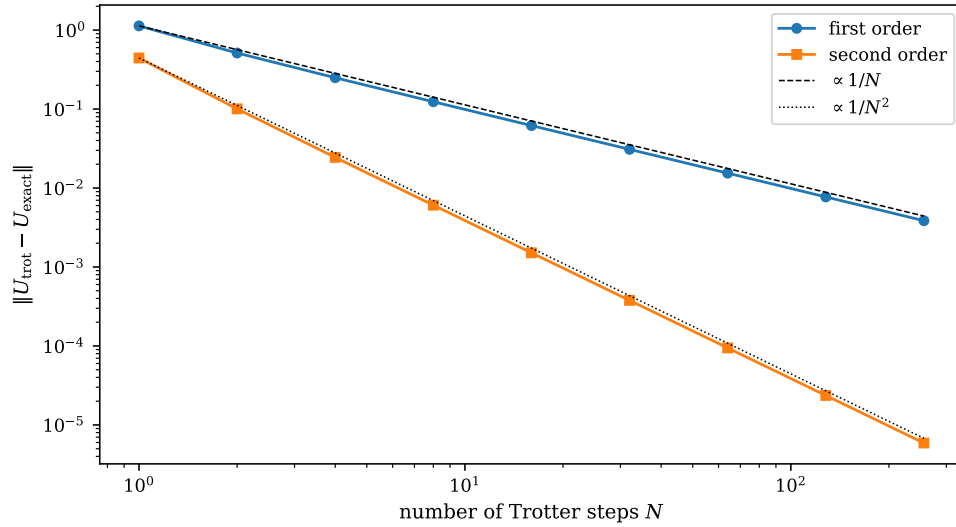
Fig. 6.2 Spectral-norm error \|U_{\text{trot}} - U_{\text{exact}}\| of the Lie-Trotter product (6.72) and of the Strang splitting (6.73) for a single qubit with \hat{H} = \sigma_x + \sigma_z propagated to t = 1 , against the number of Trotter steps N , on logarithmic scales. The two straight reference lines are e_1(1)/N and e_2(1)/N^2 , anchored on the respective one-step errors. Both sequences settle onto their asymptotic slopes of -1 and -2 after a couple of halvings of the step, and at N = 256 the symmetrised scheme is nearly three orders of magnitude more accurate than the unsymmetrised one.
