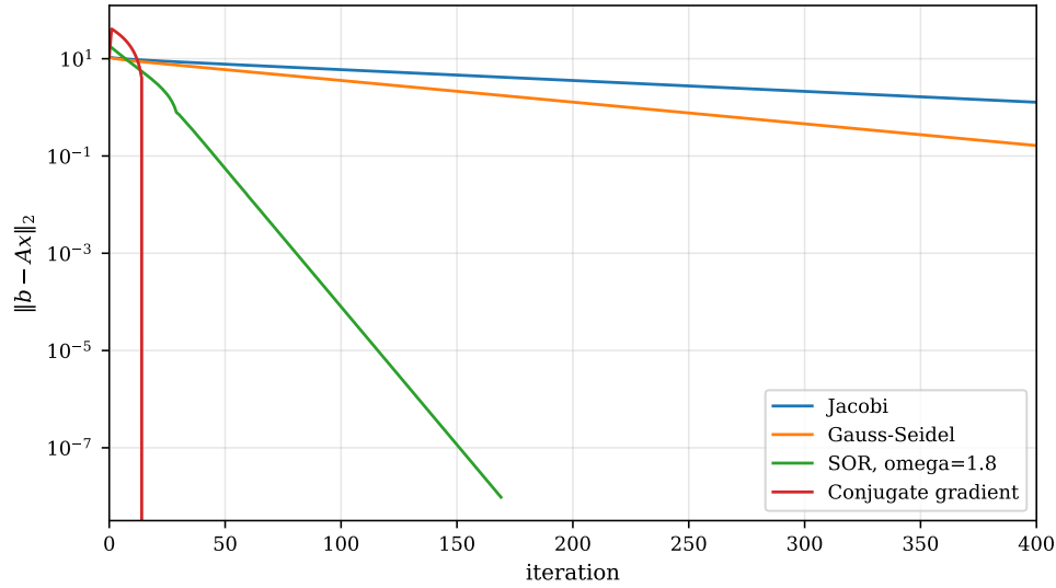
Fig. 1.3 Residual norm \|b - Ax_k\|_2 against the iteration index for the four solvers of Sections 1.17 and 1.18, applied to the discretised second derivative of Eq. (1.30) with n = 30 interior points, right-hand side b_i = 2 and starting vector x_0 = \mathbf{0} . The ordinate is logarithmic, so the straight lines of Jacobi, Gauss-Seidel and successive over-relaxation display the geometric decay \|r_k\| \sim \rho^k characteristic of a stationary iteration, with \rho the spectral radius of its iteration matrix. Over-relaxation with \omega = 1.8 loses roughly one decade every fifteen sweeps and reaches the tolerance 10^{-8} after 170 iterations, whereas Jacobi needs 4030 and Gauss-Seidel 1616; the conjugate gradient curve falls vertically out of the frame after 16 steps, having reached the rounding level.
