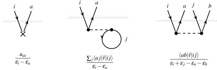
Fig. 9.5 The first-order wave function, Eq. (9.41): the three open diagrams with one vertex, each divided by the denominator of the lines crossing the cut (dotted) above it. The first two are the single excitations, with the Fock-matrix vertices of Fig. 6.6; the third is the double excitation, with the pair-creation vertex of Fig. 7.6. In a Hartree-Fock basis the first two cancel each other.
