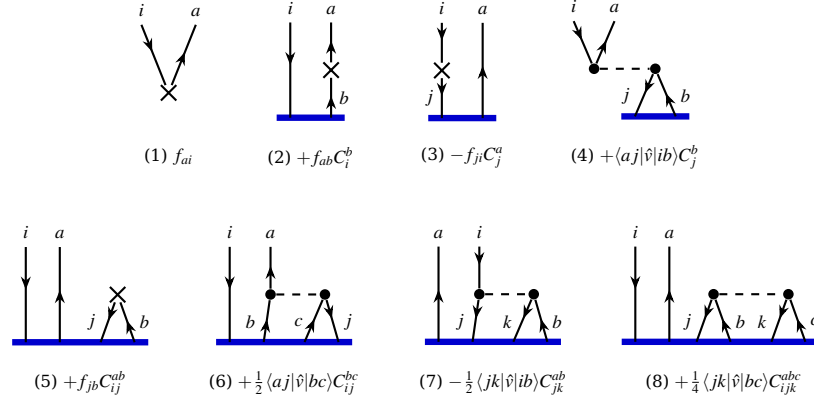
Fig. 5.6 The eight diagrams of the singles equation, Eq. (5.48), with the open lines a (particle) and i (hole) of the bra \langle\Phi_i^a| at the top. Diagrams (1)–(4) involve no amplitude or a C_1 bar, (5)–(7) a C_2 bar, (8) a C_3 bar. The signs and factors below each diagram follow from the four rules of the text.
