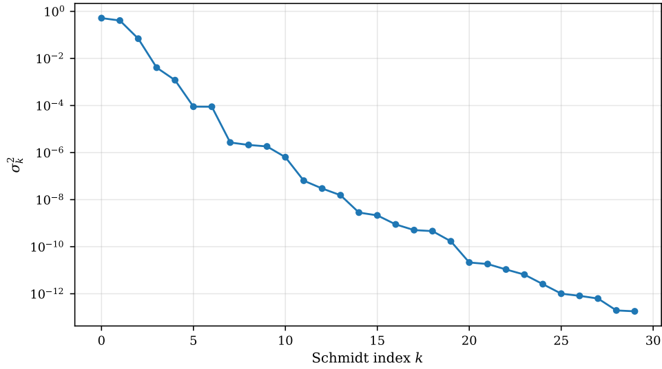
Fig. 1.6 Schmidt weights \sigma_k^2 of the pairing-model ground state (12 levels, 6 pairs, \delta = 1 , g = 0.5 ) across the cut separating the lowest six levels from the highest six, plotted logarithmically against the Schmidt index k for the thirty largest of the 64 values. The first two weights, 0.5169 and 0.4085, are of the same order and together account for 92.5% of the norm; thereafter the spectrum falls by roughly half a decade per index, reaching 10^{-6} by k = 8 and 10^{-12} by k = 25 . The small plateaux, for instance the pair of equal weights 8.9 \times 10^{-5} at k = 5 and k = 6 , are degeneracies imposed by the symmetry of the Hamiltonian.
