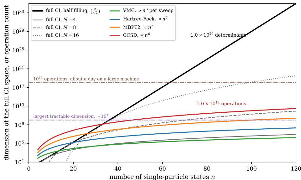
Fig. 22.1 The exponential wall, and what the five bargains buy. The dimension of the full CI space is plotted against the number of single-particle states n on a logarithmic vertical axis, for half filling (the heavy black curve, \binom{n}{n/2} ) and at fixed particle numbers N = 4, 8 and 16 (grey); against these are drawn the operation counts of the polynomial methods, \mathcal{O}(n^3) for a variational Monte Carlo sweep, \mathcal{O}(n^4) for Hartree-Fock, \mathcal{O}(n^5) for MBPT2 and \mathcal{O}(n^6) for CCSD. The two dash-dotted horizontal lines mark a dimension of 10^{10} , about the largest an iterative diagonalisation reaches, and 10^{18} operations, roughly a day on a large machine. Prefactors have been dropped and a dimension is not a floating-point operation, so only the slopes and the gap between the two families of curve carry meaning.
