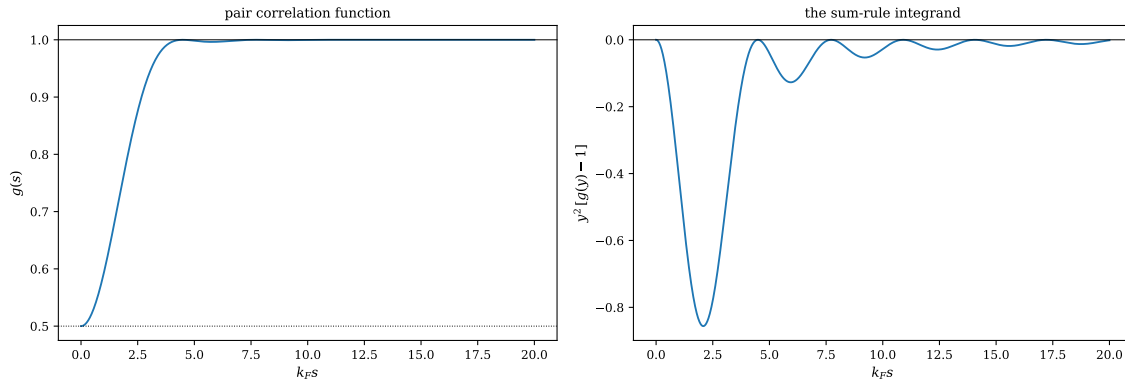
Fig. 8.3 Left: the Hartree-Fock pair correlation function (8.39) of the unpolarised electron gas against the scaled separation y = k_F s , with the uncorrelated value g = 1 and the coincidence value g(0) = \frac{1}{2} marked by the solid and dotted horizontal lines. Right: the integrand y^2[g(y) - 1] of the sum rule (8.40), whose integral over all y must be -3\pi/4 . The hole is deepest at coincidence and has essentially healed by y \simeq 4 , where g = 0.9962 , but the integrand carries a long oscillatory tail decaying only as y^{-2} : the range plotted here accounts for 95% of the sum rule, and the remaining 5% lies beyond k_F s = 20 .
