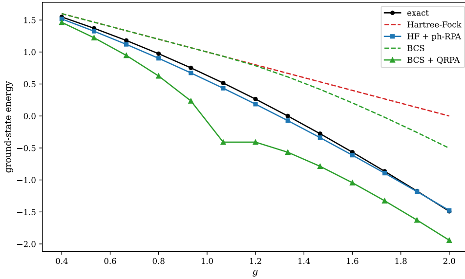
Fig. 7.10 Ground-state energy of the pure pairing model, N = L = 4 and \xi = 1 , in the four treatments of this chapter over 0.4 \leq g \leq 2.0 : exact, Hartree-Fock, Hartree-Fock plus particle-hole RPA, BCS, and BCS plus QRPA. Hartree-Fock is the straight line 2 - g , and the BCS curve, which lies on top of it below g_c = 1.07 , leaves it there. The particle-hole RPA curve is almost indistinguishable from the exact one across the whole range, whereas BCS plus QRPA lies far below it everywhere, by 0.45 at g = 2 . The kink in the QRPA curve just above g = 1 is the pairing instability of the normal vacuum. The figure is the graphical form of Table 7.6.
