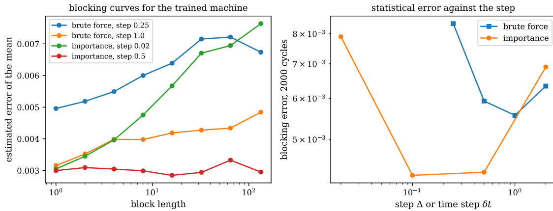
Fig. A.17 Left: blocking curves, the naive error of the mean after successive pairwise averagings of the local-energy series, for the brute-force and the importance-sampled walk at two steps each; the plateau is the true statistical error. Right: the blocking error of the energy for 2000 cycles against the step of each sampler.
