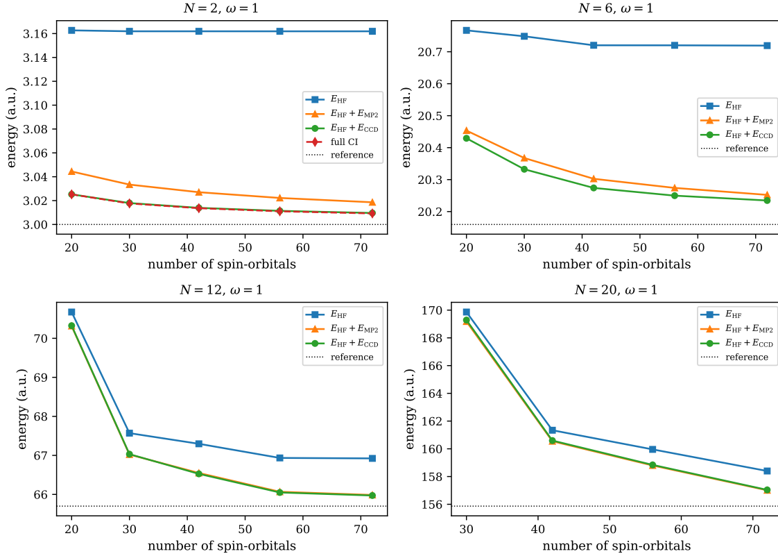
Fig. A.14 Convergence with the basis at \omega = 1 for N = 2, 6, 12 and 20 : the Hartree-Fock energy, Hartree-Fock plus MP2 and Hartree-Fock plus CCD against the number of spin-orbitals (four to eight oscillator shells), with full CI for N = 2 and the reference energy of each dot as a dotted line (Taut's exact result for N = 2 , the diffusion Monte Carlo energies of Ref. [56] otherwise). For N = 2 the CCD and full CI curves are indistinguishable on this scale; for N = 12 and N = 20 so are the MP2 and CCD curves.
