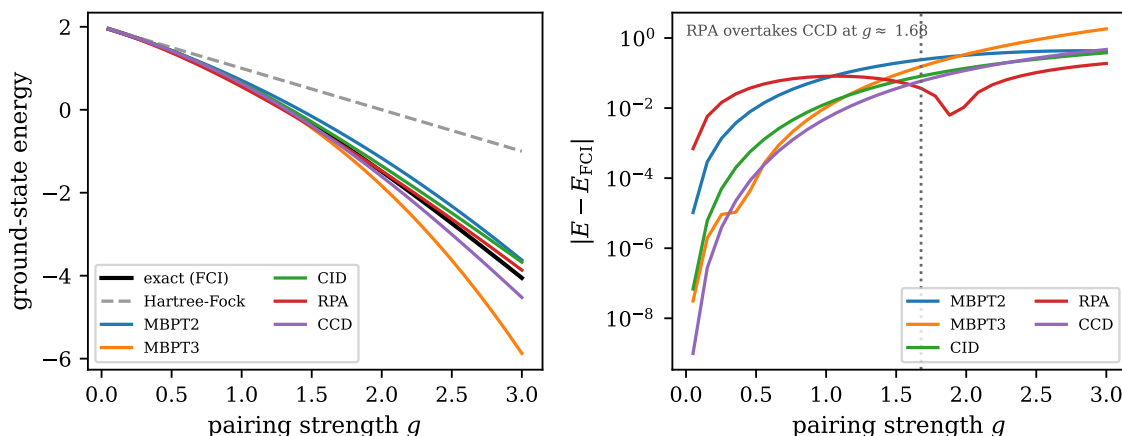
Fig. 22.3 The ordering of the methods is not stable in the coupling: the pairing model with four doubly degenerate levels and four particles, over thirty couplings from g = 0.05 to g = 3 . Left, the ground-state energy itself, with the exact diagonalisation in black and the Hartree-Fock reference as a grey dashed line; right, the absolute error |E - E_{\text{FCI}}| of each approximation on a logarithmic scale, which is the only scale on which the crossings are visible. The dotted vertical line marks g \approx 1.68 , the coupling beyond which the random-phase approximation – comfortably the worst of the five at weak coupling – is the most accurate method available.
