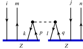
Fig. 7.9 The quadratic term \mathbf{ZBZ} of the Riccati equation (7.31): the pair-annihilation vertex joins one particle-hole pair from each of two amplitude bars, leaving one pair of each bar open. It is the ring part of the \frac{1}{2}\hat{T}_2^2 term of coupled-cluster theory, and it has no counterpart in the linear equations of configuration interaction.
