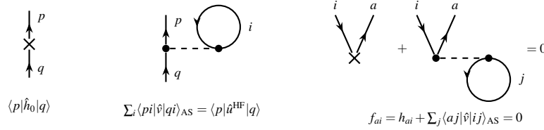
Fig. 6.6 Left and middle: the two open diagrams with one line in and one line out, the bare one-body vertex and the bubble insertion. Their sum is the Fock matrix f_{pq} , Eq. (6.96); the bubble insertion alone is the Hartree-Fock potential \hat{u}^{HF} . Right: the Hartree-Fock condition, Eq. (6.97) – the same two diagrams with the line in taken as a hole i and the line out as a particle a , required to add up to zero.
