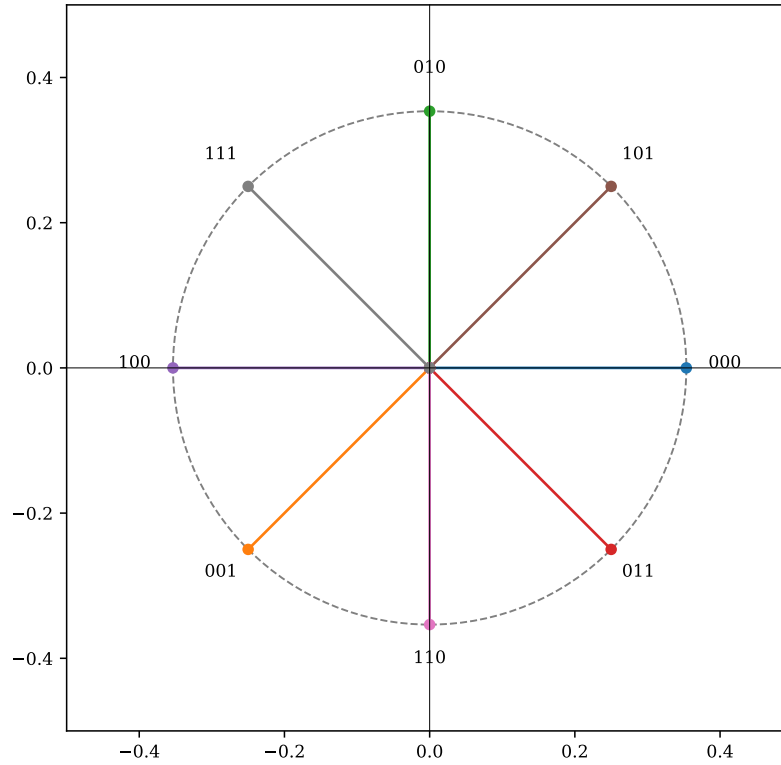
Fig. 20.3 The eight amplitudes of \text{QFT}_8|101\rangle , drawn as vectors in the complex plane and labelled by the output basis state |k\rangle they belong to. Every one of them has the same modulus 1/\sqrt{8} = 0.3536 , marked by the dashed circle, and the phase of |k\rangle is 2\pi \times (5k/8 \bmod 1) , which is the Fourier kernel of Eq. (20.3) with x = 5 . Since 5 and 8 have no common factor the eight vectors occupy the eight eighth-roots of unity exactly once each, reached in the order 0, 5, 2, 7, 4, 1, 6, 3 as k runs from 0 to 7. Computed by qpe.py .
