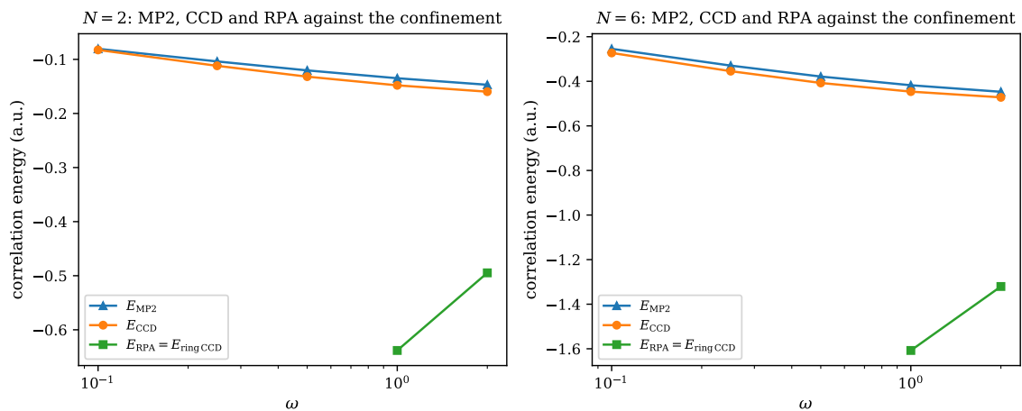
Fig. A.15 Correlation energies against the trap frequency for N = 2 (left) and N = 6 (right) in the 42-orbital basis: MP2, CCD, and the RPA, which equals ring-CCD wherever it exists. In the shaded region the symmetry-conserving Hartree-Fock determinant is RPA-unstable, the RPA equation has imaginary roots and the ring series diverges, while CCD remains finite.
