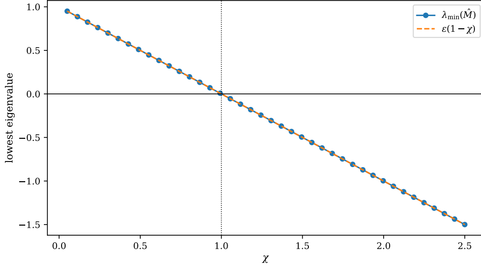
Fig. 6.4 Lowest eigenvalue of the Hartree-Fock stability matrix (6.85) for the Lipkin model with N = 4 , \varepsilon = 1 and W = 0 , built numerically from the Hamiltonian in the determinant basis at forty values of the coupling \chi , compared with the analytic result \varepsilon(1 - \chi) of Eq. (6.93). The horizontal line marks zero and the dotted vertical line the critical coupling \chi = 1 . The numerical eigenvalues lie on the analytic straight line to plotting accuracy and cross zero exactly where the deformed minimum of Figure 6.3 appears.
