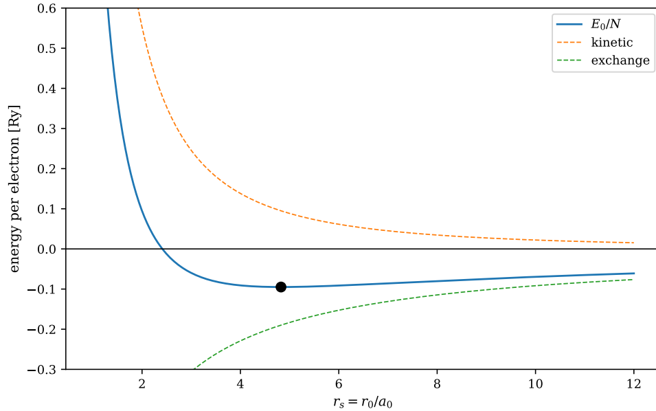
Fig. 6.11 Hartree-Fock energy per electron of the three-dimensional electron gas, Eq. (6.133), in Rydberg and against the density parameter r_s = r_0/a_0 , decomposed into the kinetic term 2.21/r_s^2 and the exchange term -0.916/r_s . The two contributions carry opposite signs and different powers of the density, so their sum turns over; the filled circle marks the minimum at r_s = 4.83 , where E_0/N = -0.0949 Ry = -1.29 eV. The total crosses zero at r_s = 2.41 and the well is very shallow, the energy staying within 5% of its minimum over the whole interval 4 \leq r_s \leq 6 .
