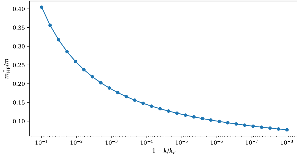
Fig. 6.10 Hartree-Fock effective mass (6.131) of the electron gas at r_s = 4 , in units of the bare mass, evaluated at thirty momenta approaching the Fermi surface from below and plotted against 1 - k/k_F on a logarithmic scale that runs from 10^{-1} on the left to 10^{-8} on the right, so that the Fermi surface lies at the right-hand edge. The ratio falls monotonically from 0.40 to 0.076, and it does so like the reciprocal of \ln(1 - k/k_F) : eight decades in the distance to the Fermi surface cost only a factor of five in m^* .
