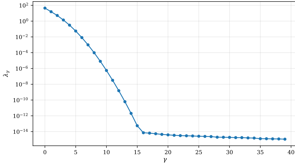
Fig. 1.8 The forty largest eigenvalues \lambda_\gamma of the two-body matrix (1.119) in the composite pair index, on a logarithmic scale, for the basis of twelve Gaussians of Section 1.29, for which the pair index runs over 144 values. The spectrum falls from \lambda_0 = 44.7 to 10^{-14} within sixteen indices and is flat thereafter: the tail beyond \gamma \approx 16 sits at the rounding level 10^{-14} , roughly \lambda_0 times the machine epsilon, and carries no information. The numerical rank of the interaction is therefore about sixteen, an order of magnitude below the 144 that naive counting of pair indices would suggest.
