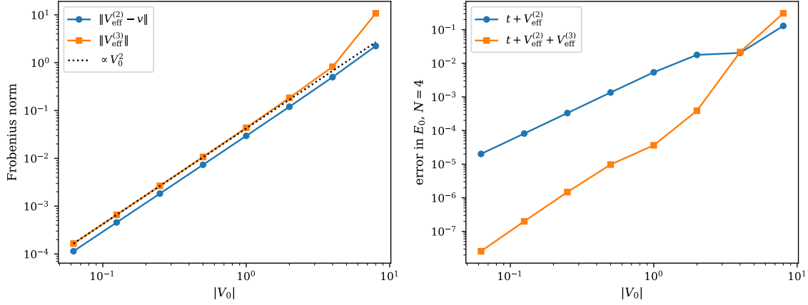
Fig. A.7 Left: Frobenius norms of the renormalisation of the two-body interaction, \|\hat{V}_{\text{eff}}^{(2)} - \hat{v}\| , and of the induced three-body interaction, \|\hat{V}_{\text{eff}}^{(3)}\| , as functions of the coupling |V_0| for n = 14 , n_P = 6 , \sigma = 1 and \Delta = 3 ; the dotted line is \propto V_0^2 . Right: the error in the four-particle ground-state energy of the model-space calculation with \hat{t} + \hat{V}_{\text{eff}}^{(2)} and with \hat{t} + \hat{V}_{\text{eff}}^{(2)} + \hat{V}_{\text{eff}}^{(3)} . Both norms follow the V_0^2 line at weak coupling; at V_0 = -4 the three-body term no longer improves the four-particle energy and at V_0 = -8 it makes it worse.
