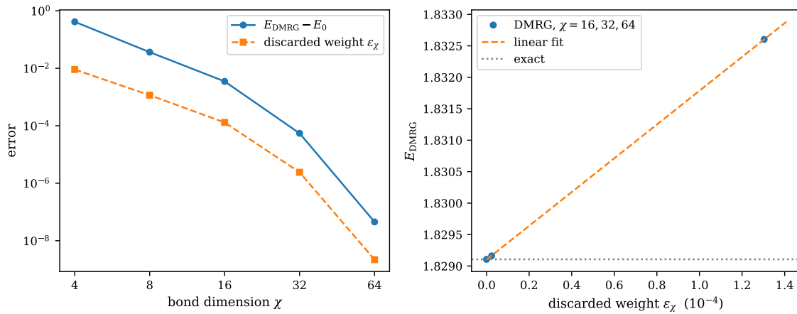
Fig. 11.6 Convergence of the DMRG for the pairing plus particle-hole model, eight levels, eight particles, g = 1 , f = 0.5 . Left: the energy error against the bond dimension, on a logarithmic scale. Right: the energy against the largest discarded weight of the final sweep for \chi = 16, 32 and 64 ; the dashed line is a straight-line fit through the three points, and its intercept at \varepsilon_\chi = 0 is the extrapolated energy. The dotted horizontal line is the exact energy.
