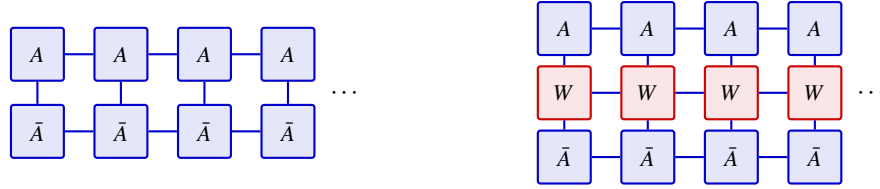
Fig. 11.3 Left: the norm \langle \Psi | \Psi \rangle of a matrix product state as a closed diagram; one column of it is the transfer matrix of Eq. (11.14). Right: the expectation value \langle \Psi | \hat{H} | \Psi \rangle with the Hamiltonian written as the matrix product operator of Section 11.3, a row of tensors W with two physical legs each, sandwiched between the state and its conjugate. Both diagrams are contracted column by column, never row by row.
