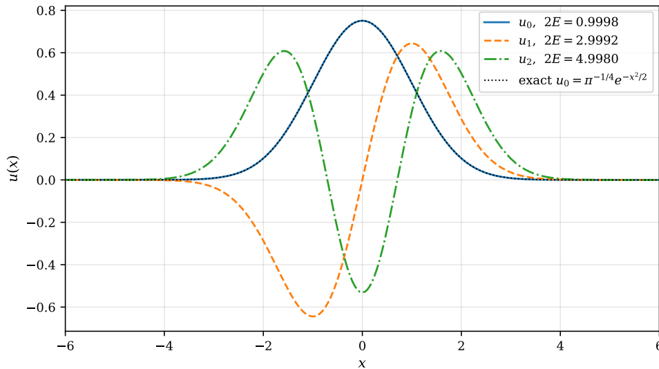
Fig. 1.5 The three lowest eigenfunctions u_n(x) of the harmonic oscillator obtained by diagonalising the tridiagonal matrix of Eq. (1.95) on x \in [-10, 10] with N_{\text{step}} = 400 , normalised by the trapezoidal rule (1.96) and plotted over the interval where they are appreciably different from zero. The legend gives the computed eigenvalues 2E_n , which should equal 1, 3 and 5. The dotted black curve is the analytic ground state u_0 = \pi^{-1/4}e^{-x^2/2} and is indistinguishable from the computed u_0 on the scale of the plot; the maximum pointwise deviation is 7 \times 10^{-5} .
