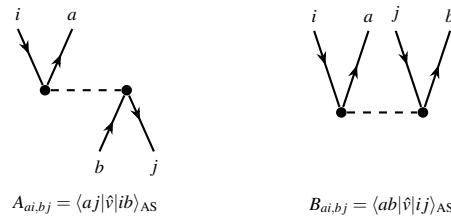
Fig. 6.8 The two blocks of the stability matrix, Eq. (6.98). Left: the particle-hole scattering diagram A , one pair in from below and one pair out above. Right: the pair-creation diagram B , two pairs out of the reference. With the excitation energies from the crosses, \Delta + A is the Tamm-Dancoff matrix and the full \hat{M} of Eq. (6.85) the matrix of the random-phase approximation.
