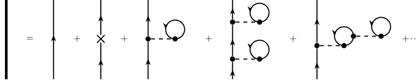
Fig. 6.7 The self-consistent field as a series. A dressed single-particle line (thick) is the bare line plus one cross, plus one bubble insertion, plus two insertions in a row, plus a bubble inside a bubble, and so on to all orders. Hartree-Fock theory sums every diagram of this kind; in a Hartree-Fock basis none of them is drawn again.
