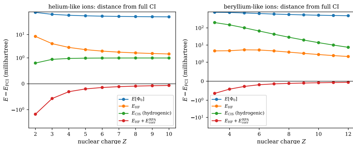
Fig. A.12 Distance from the full CI energy along the helium-like (left) and beryllium-like (right) isoelectronic sequences, in millihartree on a symmetric logarithmic scale, for the reference determinant, Hartree-Fock, CIS in the hydrogenic basis, and Hartree-Fock plus the RPA correlation energy. The reference determinant misses a roughly constant amount along each sequence; Hartree-Fock removes most of it for the beryllium-like ions and only part of it for the helium-like ones; the RPA lands below the exact answer everywhere.
