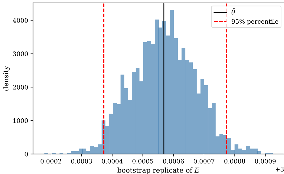
Fig. 15.8 The bootstrap distribution of the mean local energy: a normalised histogram of B = 2000 replicates, each the mean of a data set assembled by drawing 200 blocks of 1000 with replacement from the chain of 200000 local energies of Table 15.10. The solid vertical line is the estimate from the data themselves, \hat{\theta} = E = 3.000569 , and the two dashed lines are the 2.5% and 97.5% percentiles at 3.000373 and 3.000773, which lie 1.9 standard deviations either side of it. The replicates are symmetric about \hat{\theta} , with a skewness of +0.013.
