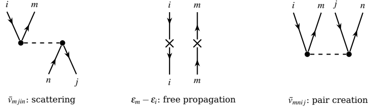
Fig. 7.6 The building blocks of the particle-hole approximations, in the Hartree-Fock basis. Left: the interaction scatters a particle-hole pair, the off-diagonal part of A . Middle: the pair propagates between two crosses carrying the Hartree-Fock orbital energies, the diagonal part of A . Right: the interaction creates two pairs, the block B ; read upside down it annihilates two.
