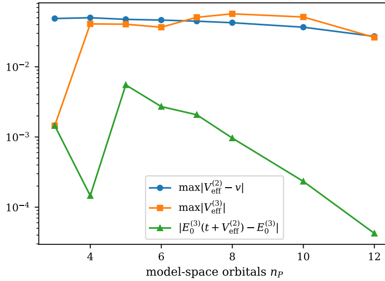
Fig. A.8 The largest matrix element of the renormalisation \hat{V}_{\text{eff}}^{(2)} - \hat{v} , the largest matrix element of \hat{V}_{\text{eff}}^{(3)} , and the error of the three-particle ground state obtained with \hat{t} + \hat{V}_{\text{eff}}^{(2)} alone, as functions of the number n_p of model-space orbitals, for n = 14 , V_0 = -2 , \sigma = 1 and \Delta = 3 above the top of each model space. At n_p = n = 14 , not shown, all three are zero to machine precision ( 10^{-12} ).
