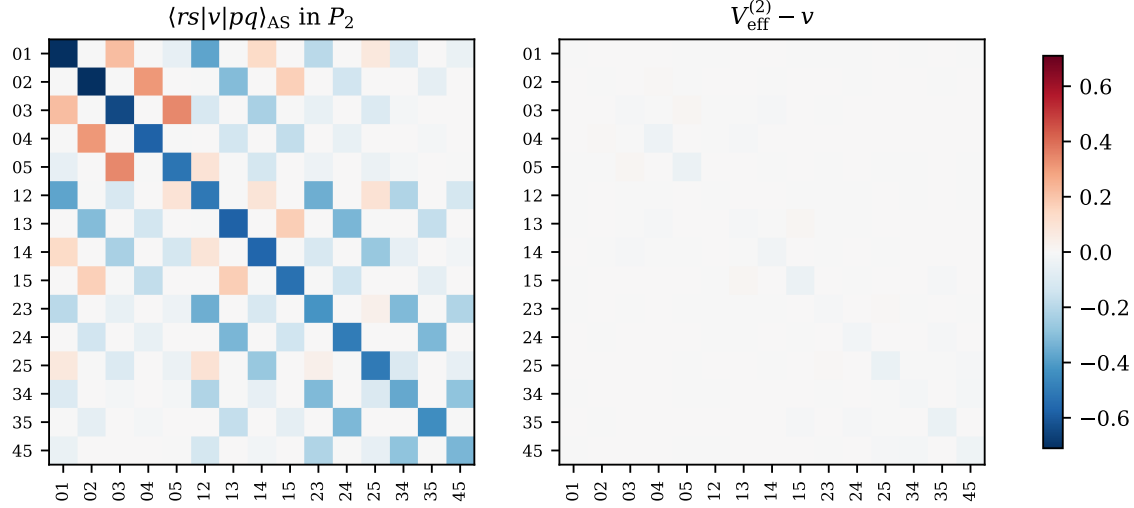
Fig. A.5 The bare interaction \langle rs|\hat{v}|pq\rangle_{AS} restricted to the two-particle model space P_2 (left) and the renormalisation \hat{V}_{\text{eff}}^{(2)} - \hat{v} produced by the Lee-Suzuki-Okubo transformation (right), on the same colour scale, for n = 14 , n_p = 6 , V_0 = -2 , \sigma = 1 and \Delta = 3 . Rows and columns are the fifteen determinants |pq\rangle of P_2 . The renormalisation is a few per cent of the bare interaction and is largest for the determinants involving the highest model-space orbitals.
