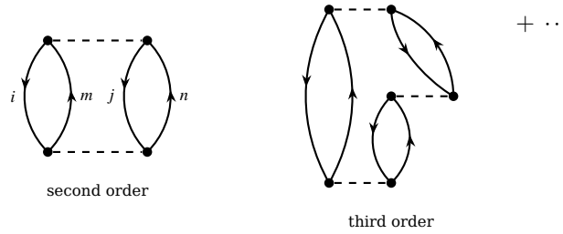
Fig. 7.8 Ring diagrams: the closed diagrams that can be built from the pair creation and annihilation vertices of B and the scattering vertex of A alone. Second order: two pairs created by one interaction and annihilated by the next, the diagram \frac{1}{2} \sum |\bar{v}_{mij}|^2 / (\epsilon_i + \epsilon_j - \epsilon_m - \epsilon_n) of second-order perturbation theory in the ring topology. Third order: one of the pairs is scattered once before both are annihilated. The RPA correlation energy is the sum of all such rings.
