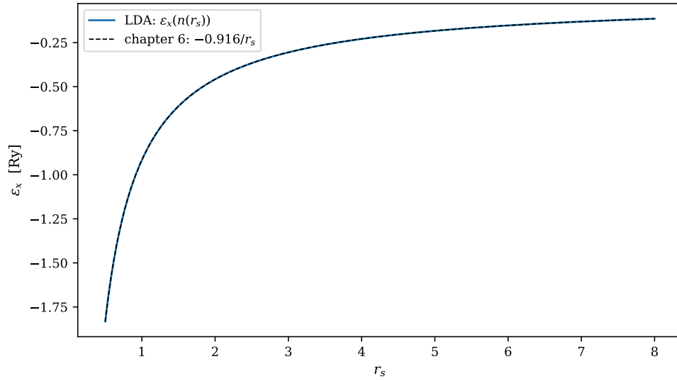
Fig. 8.2 The local exchange energy per particle \epsilon_x(n) = -\frac{3}{4}(3/\pi)^{1/3}n^{1/3} of Eq. (8.38), converted to Rydberg and plotted against the Wigner-Seitz radius r_s through n = 3/4\pi r_s^3 , together with the -0.916/r_s obtained from the filled Fermi sea in Chapter 6. The two curves are drawn separately over 0.5 \leq r_s \leq 8 and are indistinguishable at any point, the coefficients differing by 3.6 \times 10^{-4} in relative terms. The agreement is exact by construction and the figure is a check on the algebra rather than on the physics.
