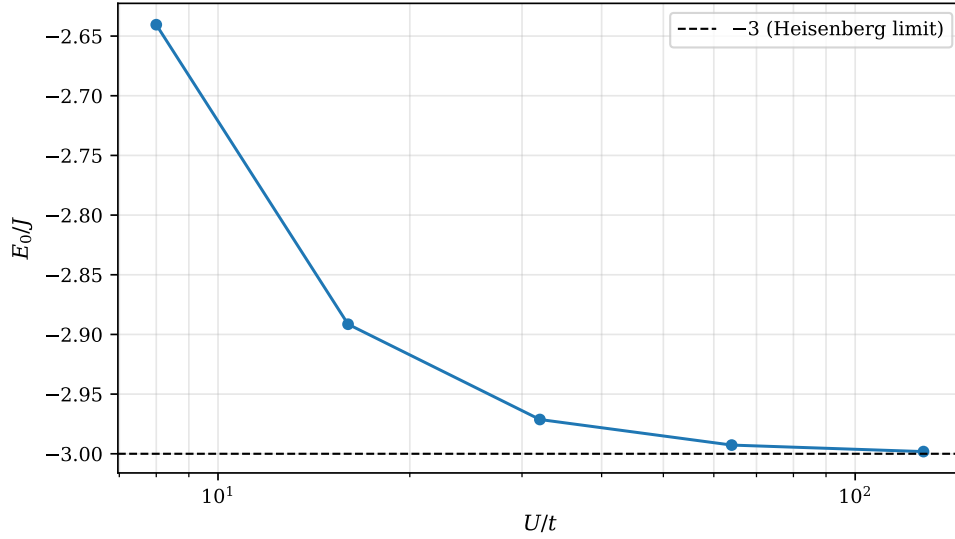
Fig. 4.6 The half-filled four-site Hubbard ring at strong coupling. Plotted is the exact ground-state energy in units of the effective exchange J = 4t^2/U , against U/t on a logarithmic scale; the dashed line is the value -3 predicted by the mapping onto the Heisenberg antiferromagnet, -2J from the exchange on the four bonds and -J from the constant -\frac{1}{4}\hat{n}_i\hat{n}_j term. The remaining deviation falls by a factor of four for every doubling of U , the signature of a leading correction of order t^4/U^3 . The five points are the rows of Table 4.5.
