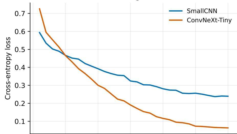
Training loss
