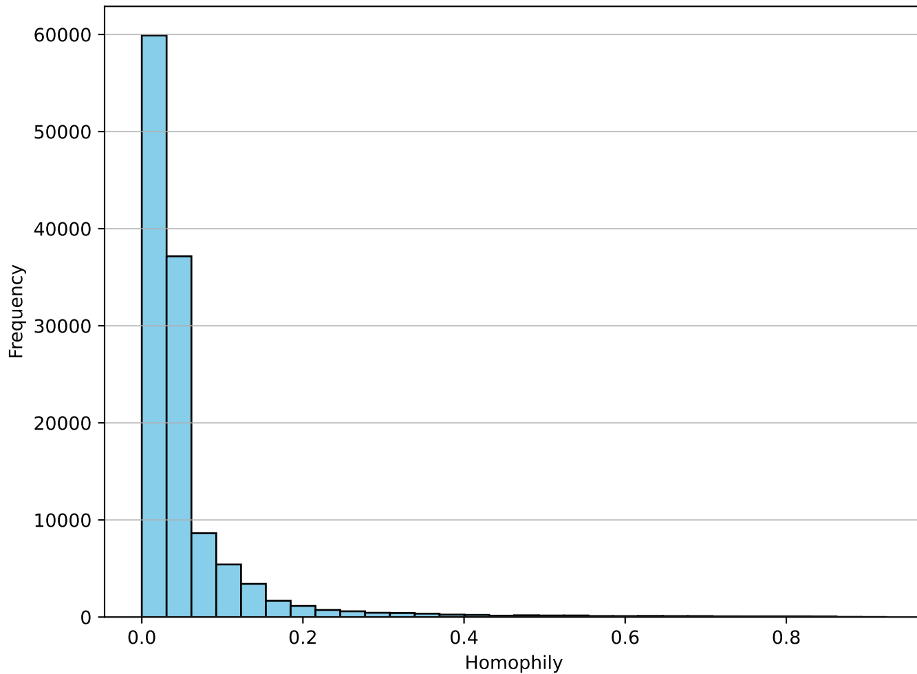
Homophily Distribution for COCO-SP
