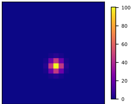
C d_I when q_E \propto V
