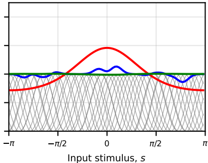
A Excitatory Mass Homeostasis
