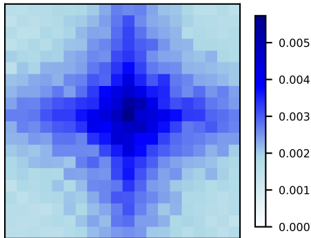
C d_I when q_E \propto V
