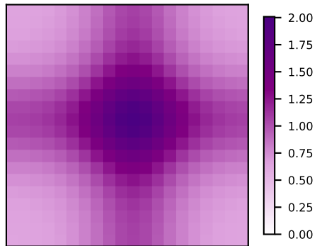
D d_I when q_I \propto V
