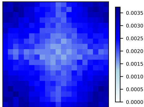
D d_I when q_I \propto V
