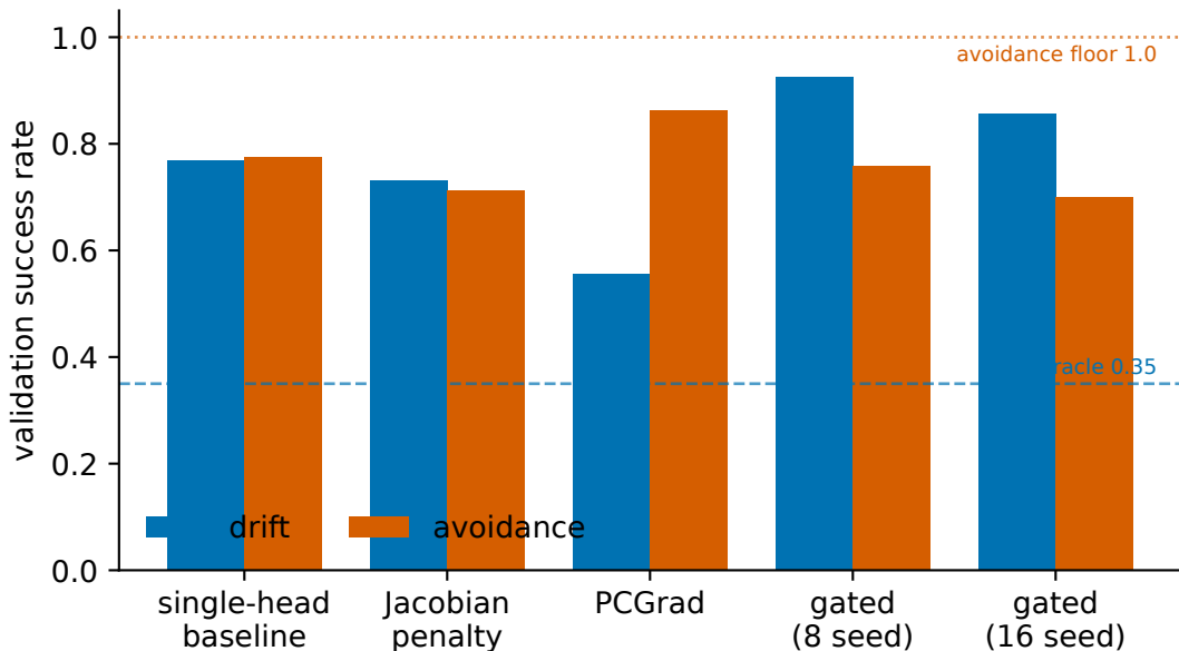
Lever elimination: only gated dual heads expand the frontier
