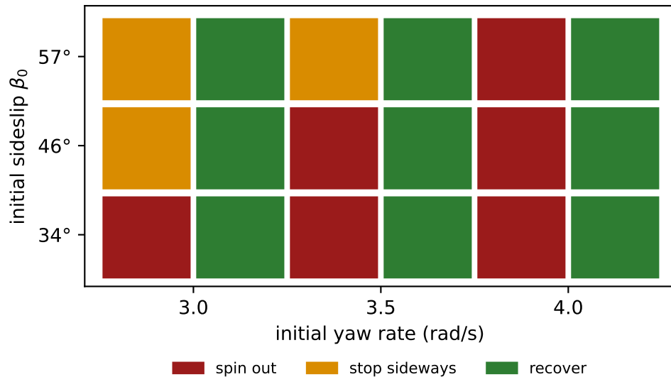
(B) After slip ( \mu = 0.5 ): brake-ESC | counter-steer (faithful Chrono)
