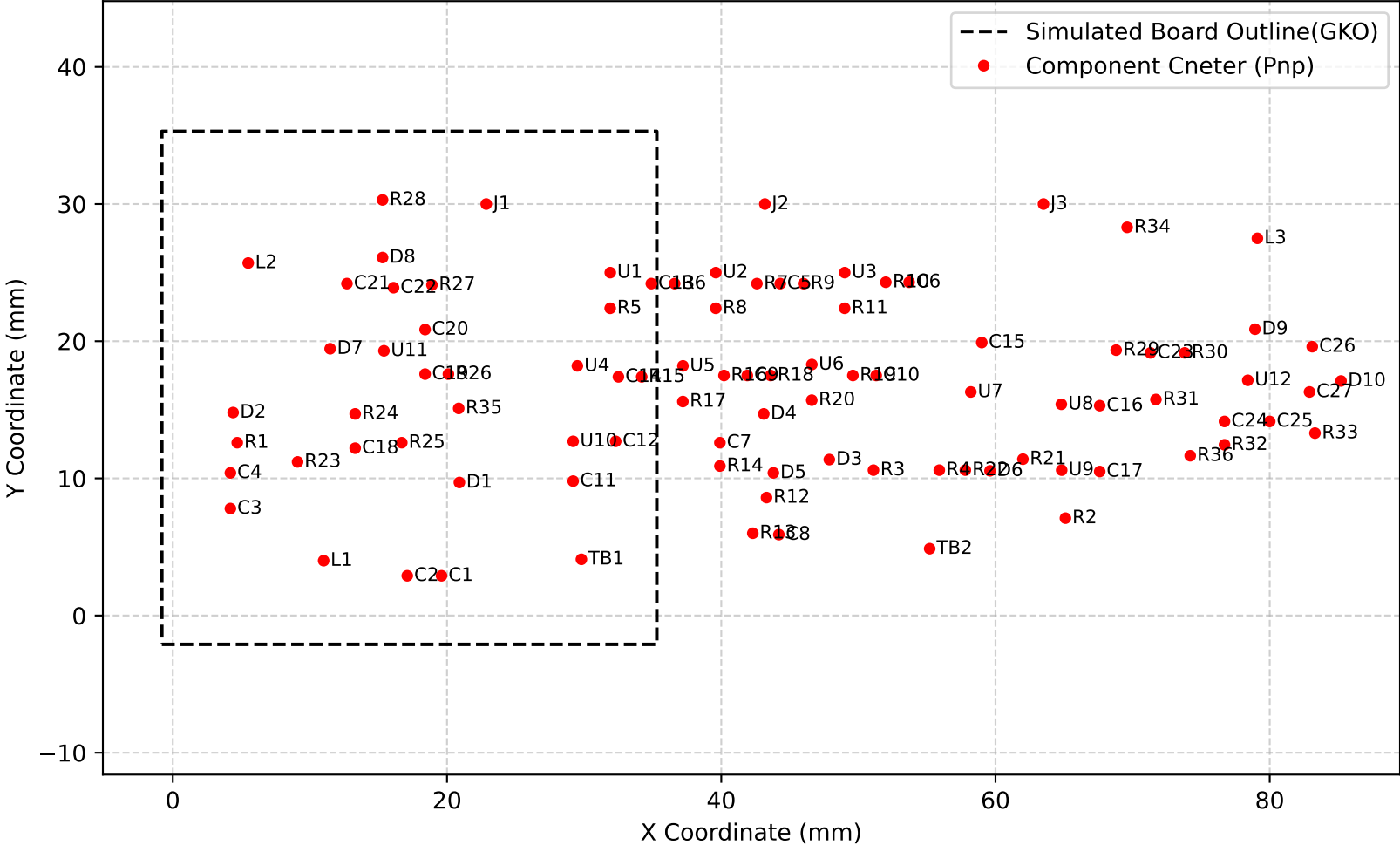
Simulated PCB Layout: Designator Location Panel 436-5002_R
