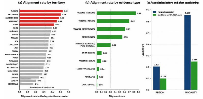
Figure 13. Equity audit of the assignment.
