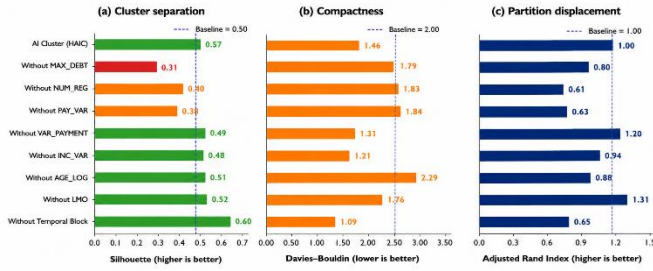
Figure 12. Allocation of variables and the temporal block.
