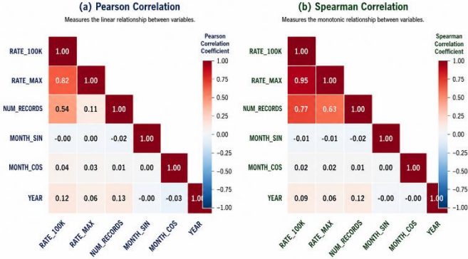
Figure 4. Correlation between the variables of interest.
