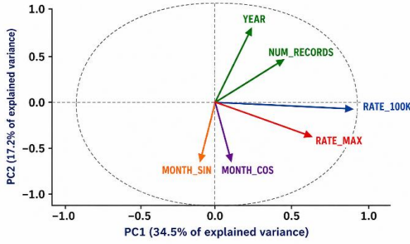
Figure 3. Loadings of the first two principal components.
