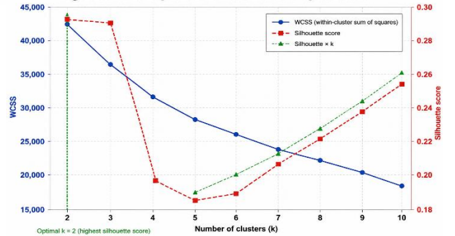
Figure 7. Selection of the number of clusters in K-Means.
