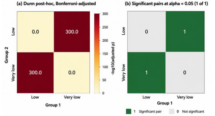
Figure 8. Multiple Dunn comparisons among groups.
