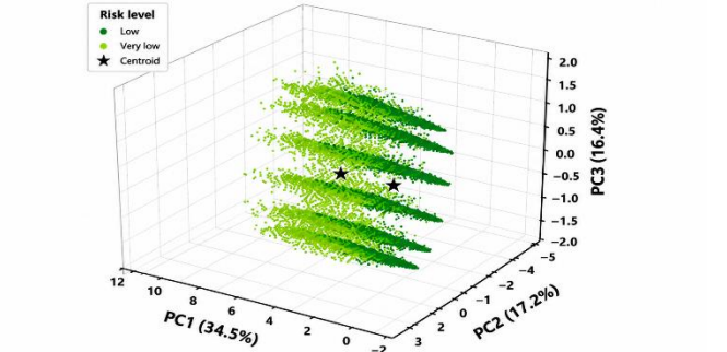
Figure 6. K-Means partition in three-dimensional representation.
