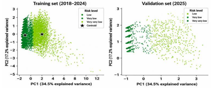
Figure 5. K-Means partition on the first two principal components.
