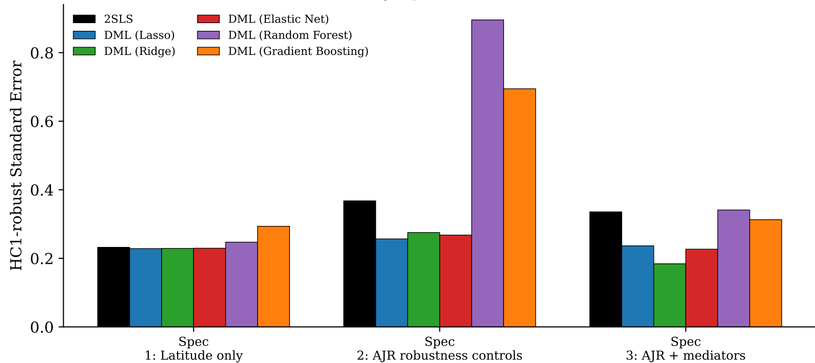
Standard Error by Specification and Estimator
